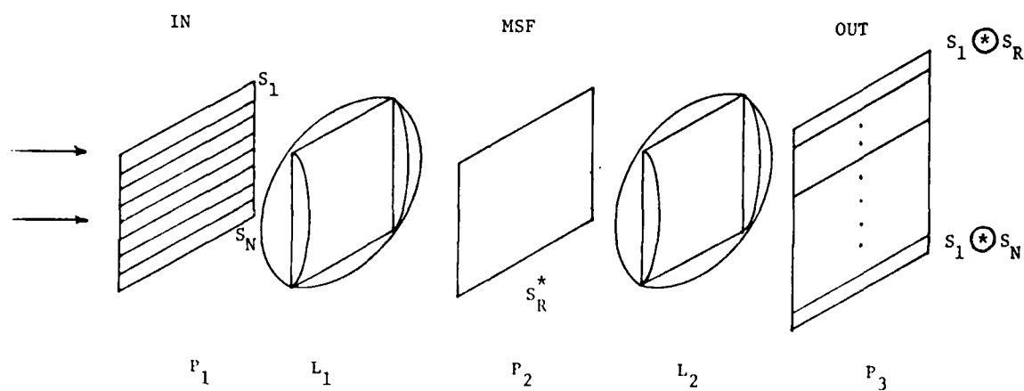
Fig. 3.4 Frequency plane optical correlator for adaptive radar processing.
