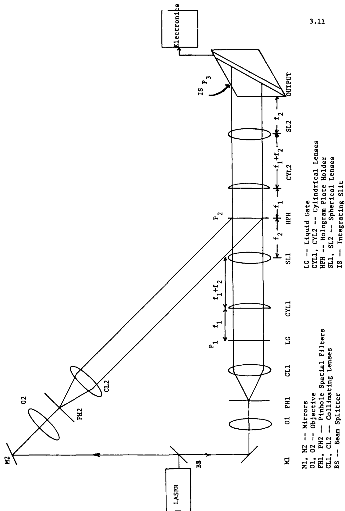
Fig. 3.5 Layout of the frequency plane correlator.
