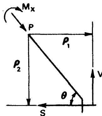
FIG a RELATION BETWEEN COMPONENTS (V,S) OF APPLIED LOAD AND INTERNAL REACTIONS ( M_x, P )
