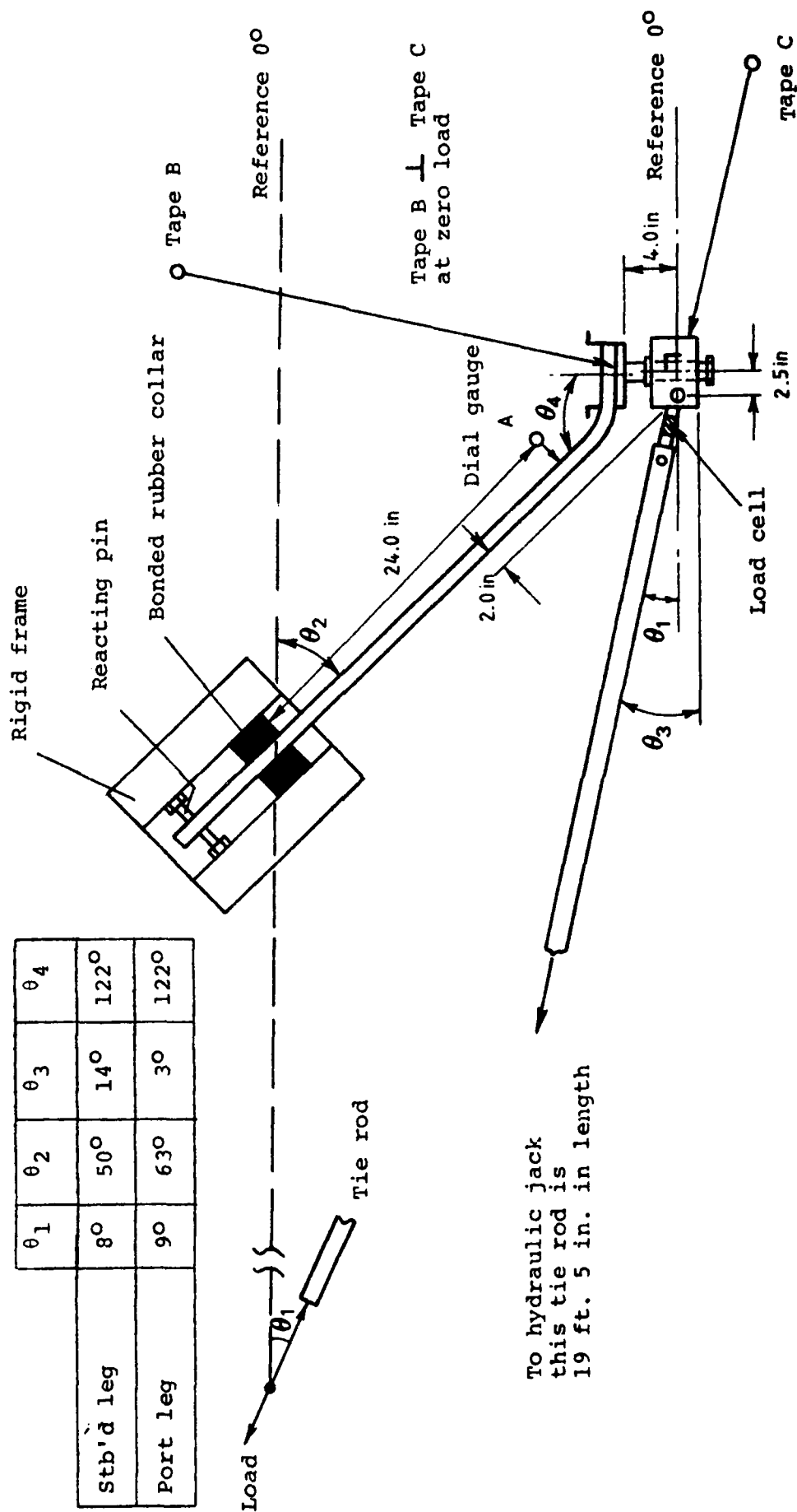
FIG. C1 LOCATIONS OF VERNIER TAPES AND DIAL GAUGES FOR VERTICAL LOAD CALIBRATION
