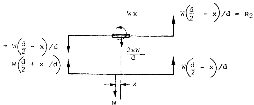
FIG. 10 PRACTICAL TORSION RIG WITH R_1 \neq R_2
