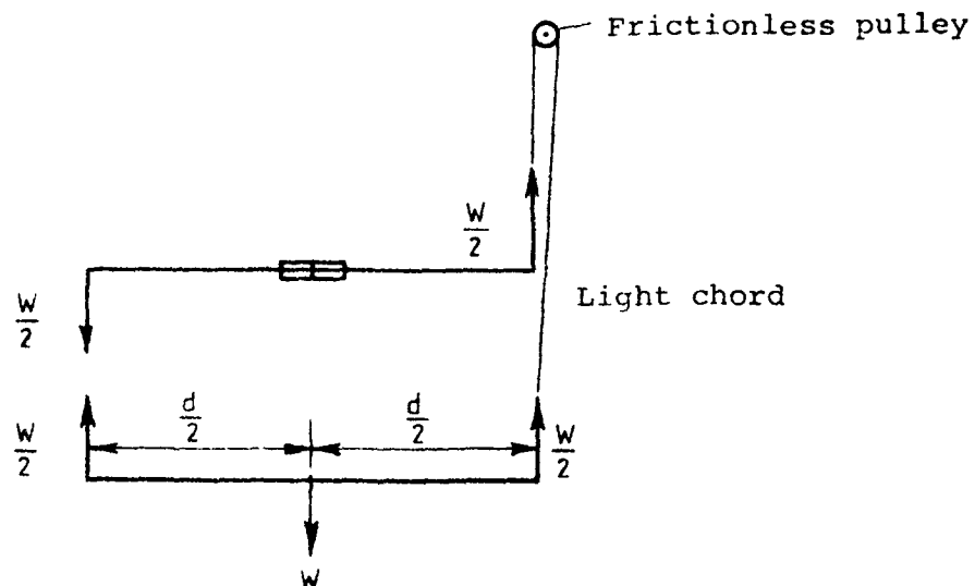
FIG. 9 IDEAL RIG TO APPLY PURE TORSION
