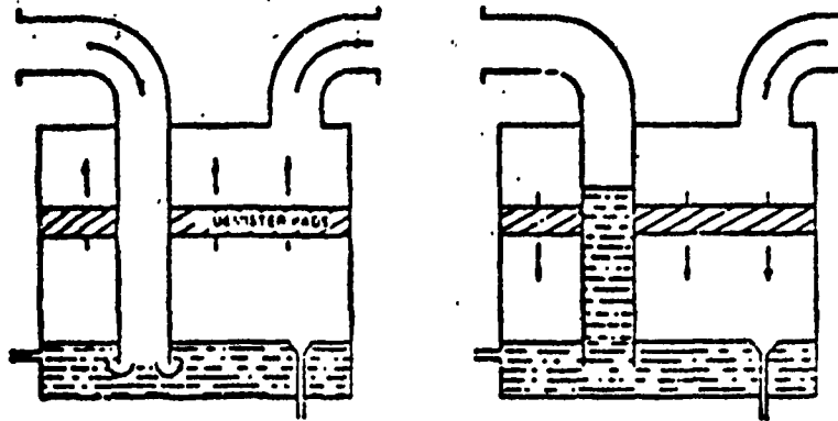
Figure 7. Deck water seal - wet type
