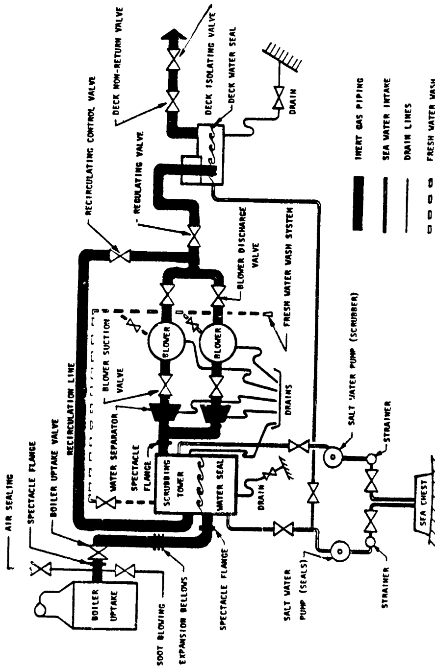
FIGURE 1 Typical Inert Gas System
