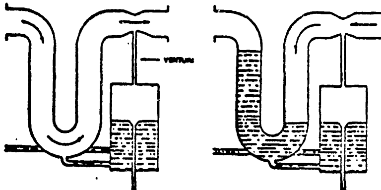
Figure 8. Deck water seal - semi dry type
