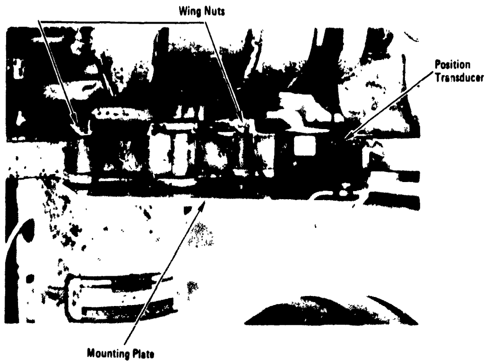
Figure 2-4. Nose Gear Steering Angle Transducer Installation
