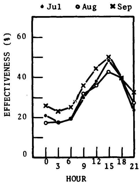
FIGURE 81. VAS EFFECTIVENESS FOR PHL RUNWAY 9/27 (CONCLUDED)
