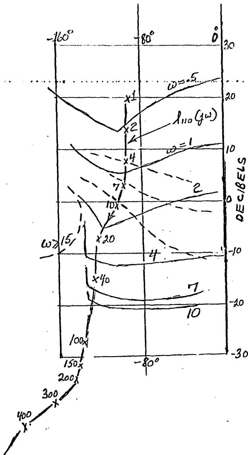
Fig. 7. Bounds on \gamma_{11}(j\omega) . Solid lines are due to | \gamma_{11} | , broken lines due to | \gamma_{12} d_{12e} |
