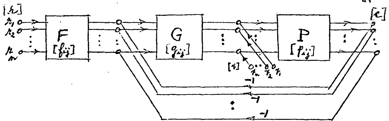
Fig. 1 Multiple input-output two matrix degree-of-freedom feedback structure c = \text{Tr} , T = [t_{ij}] , c = [c_1 \dots c_n]' , r = [r_1 \dots r_n]' .
