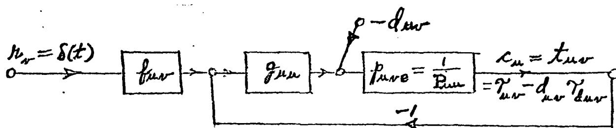
Fig. 2 Single-loop structure equivalent, for synthesis of t_{uv} ;
