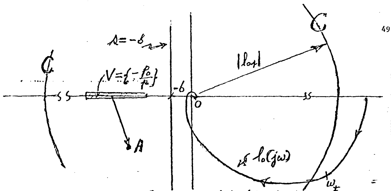
Fig. A1. Bounds on \lambda_0 : C in [0, \omega_+ ], \lambda = -b in (\omega_+, \infty) ; and a satisfactory \lambda_0(j\omega) .
