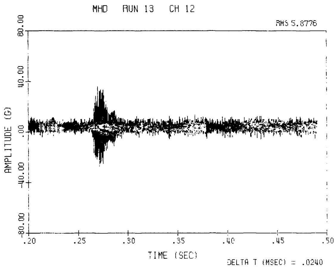
Figure 55. LWC 013, Vibration Amplitude at Beginning of Run, Channel 12
