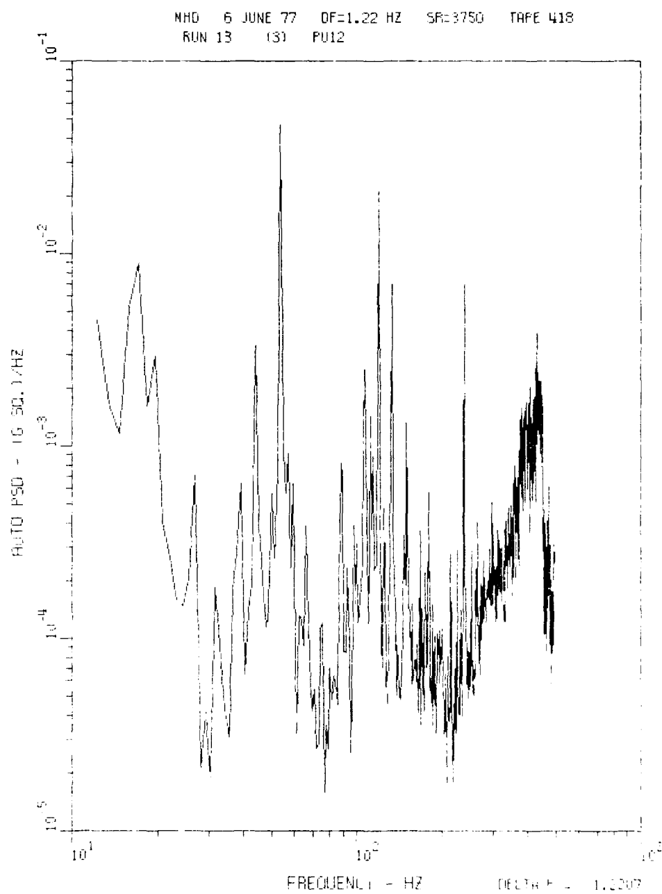
Figure 86. Channel Twelve PSD, 0-500 Hz, Run LWC 013
