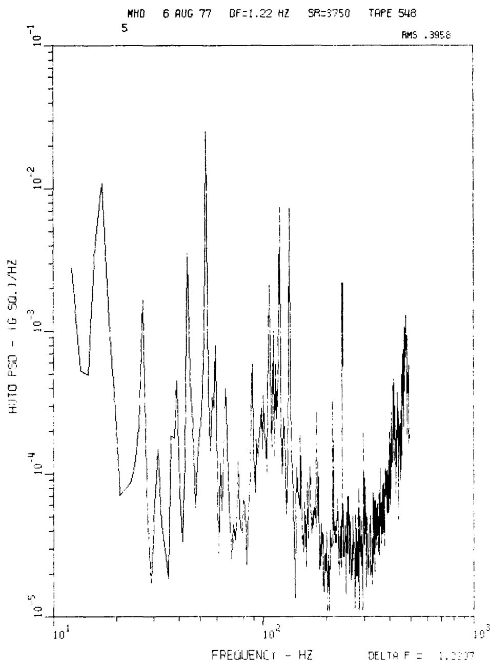
Figure 90. Channel Five PSD, 0-500 Hz, Run LWC 023
