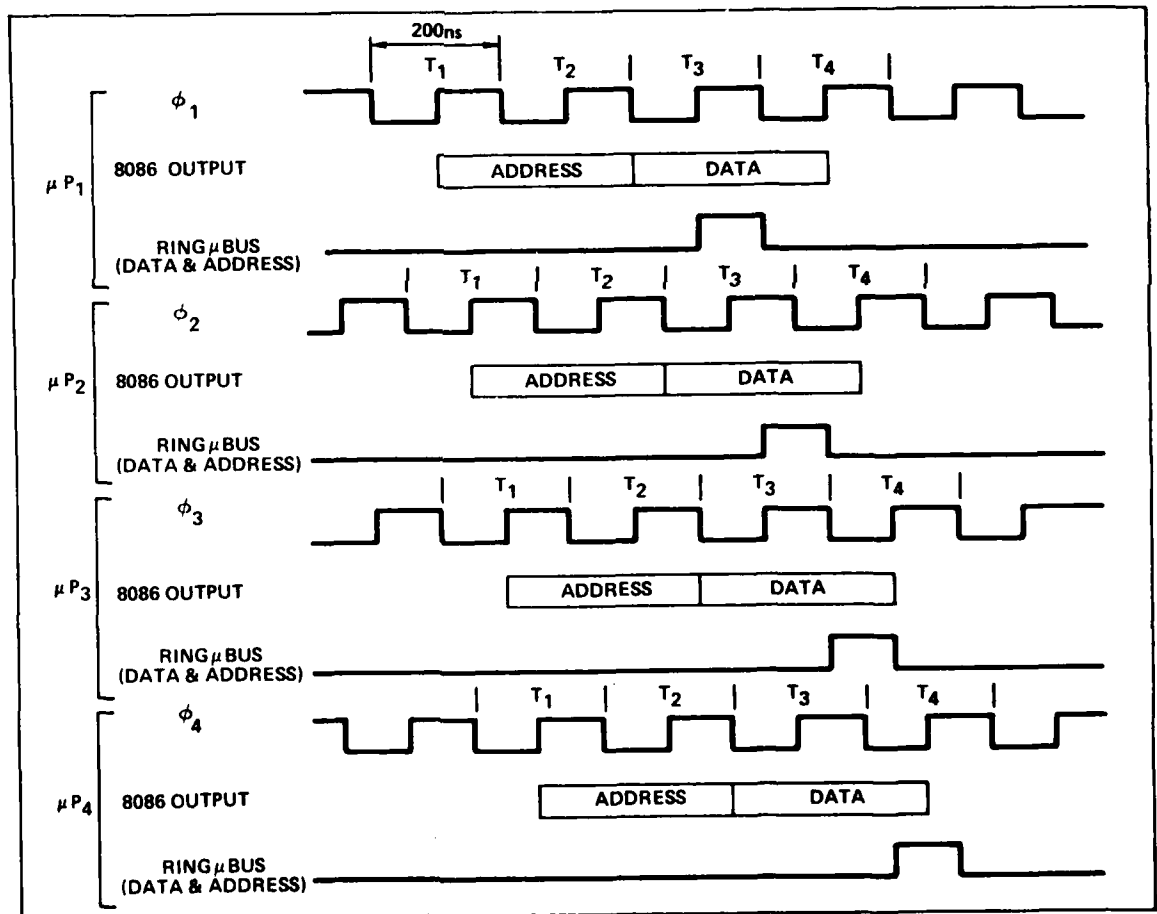
Figure 5-5 - Time-Phased Ring Bus Intel 8086 Timing Compatibility
