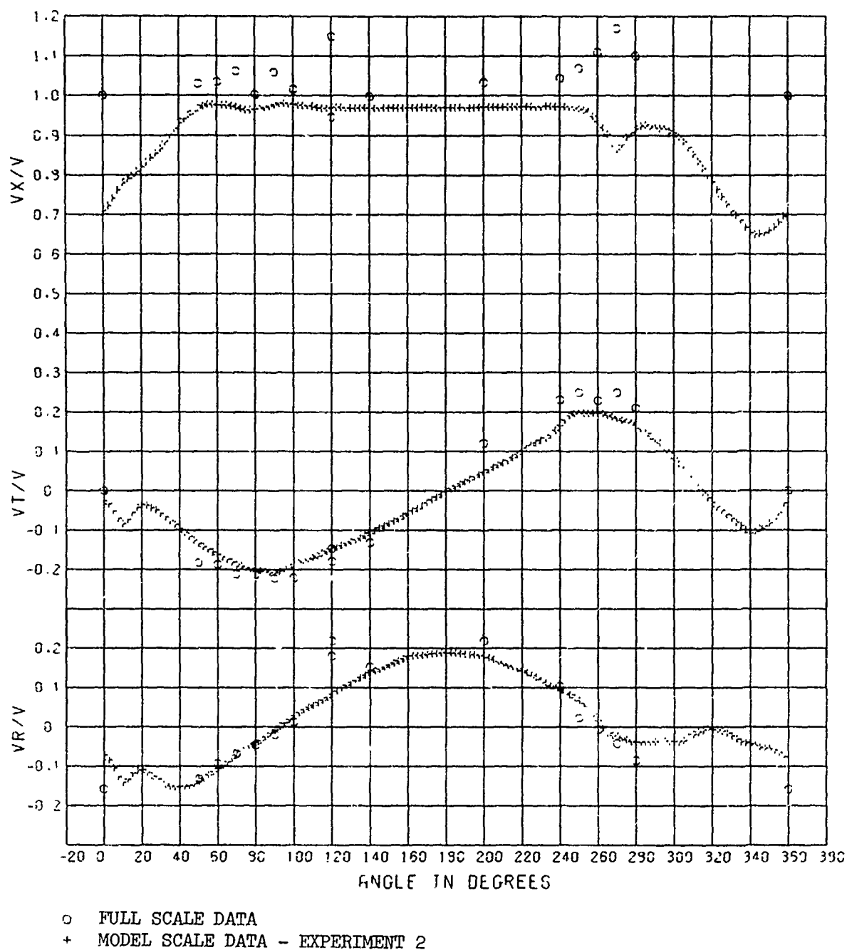
Figure 21 - Velocity Component Ratios for R/V ATHENA and Model 5366 at the Forward Rake Location ( x/L_{WL} = 0.906 ) with an Operating Propeller for the 0.917 Radius
