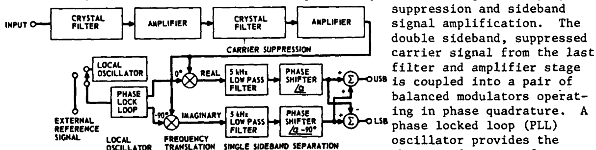
Fig. 4. Block Diagram of Band Elimination Receiver
