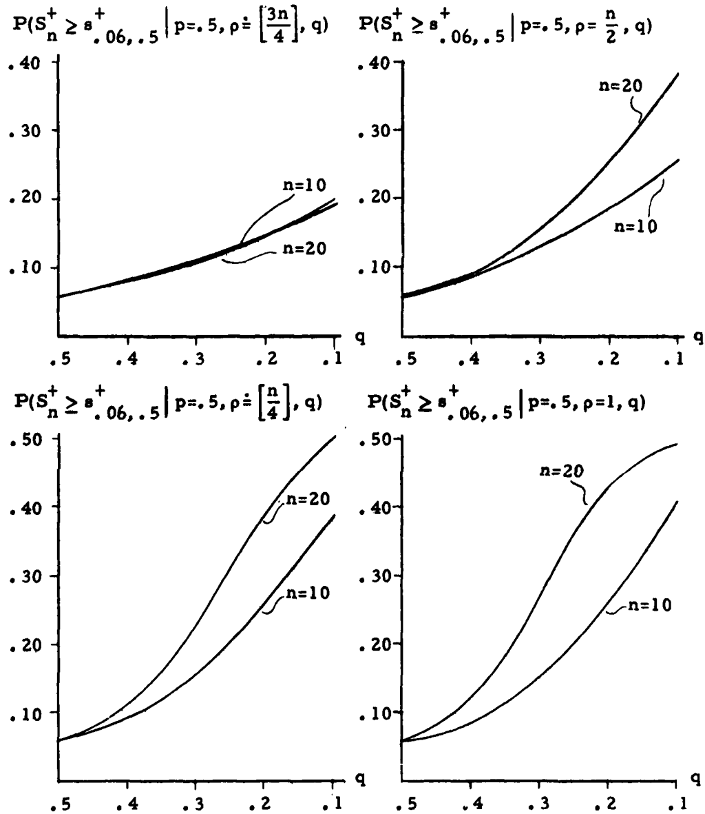
Figure 30.2. P(S_n^+ \geq s_{.06, .5}^+ \mid p=.5, \rho, q) .
