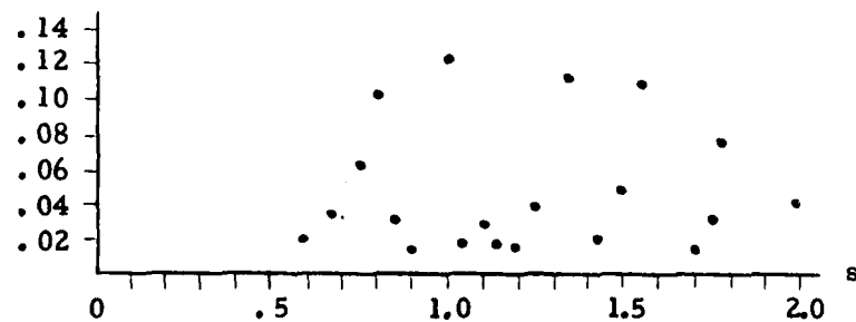
Figure 13.1 P(S_{10} = s \mid p) vs. s .
