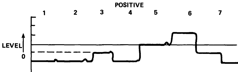
Figure 5.0-2. Test Output of Testing Metalization Pattern
