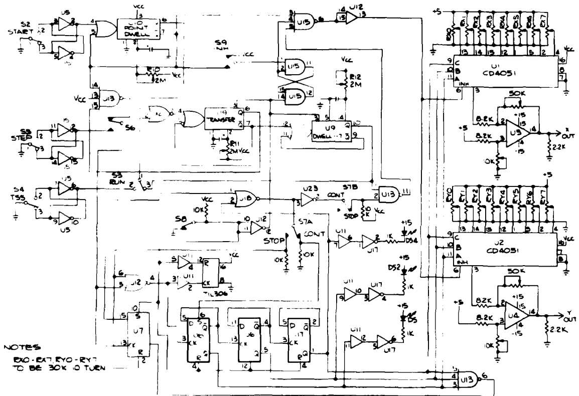
FIGURE 10 SCHEMATIC OF THE MULTI-POINT PROBE TOOLING
