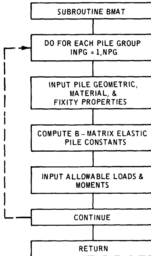
Figure 5. Flow chart of sub- routine BMAT for LMVDPILE
