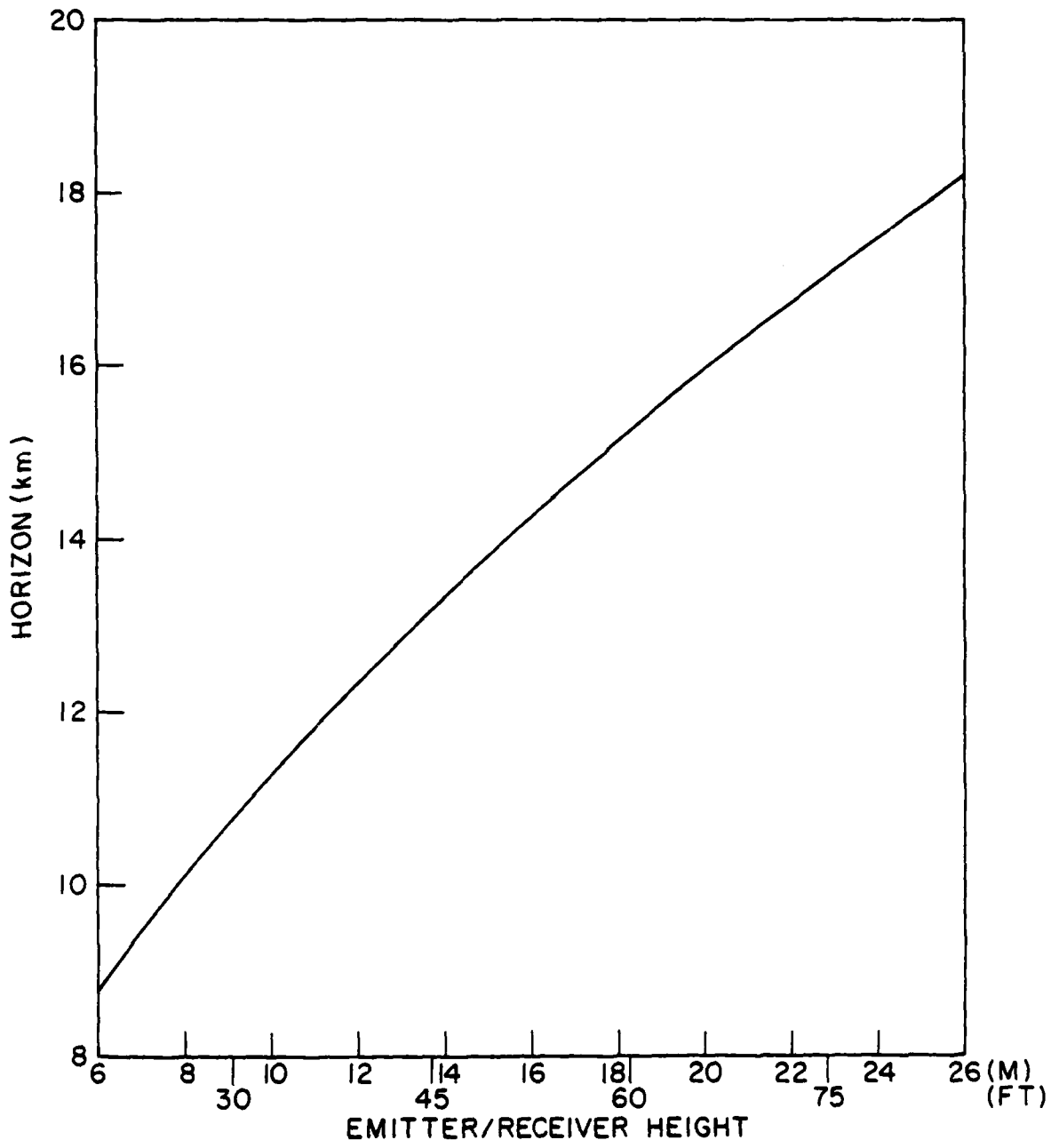
Fig. 4 — Horizon distance vs. emitter/receiver height
