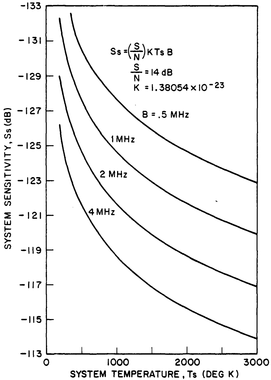
Fig. 2 - System sensitivity vs. system temperature
