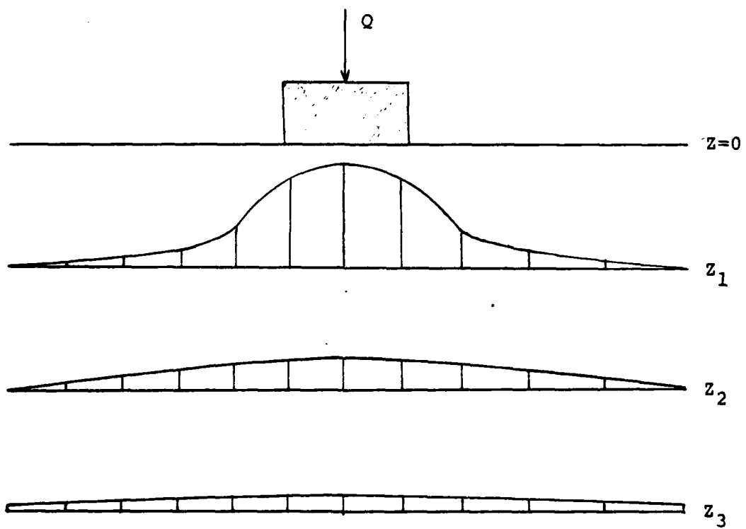
Variation of vertical stress on horizontal planes at different depths, z .
