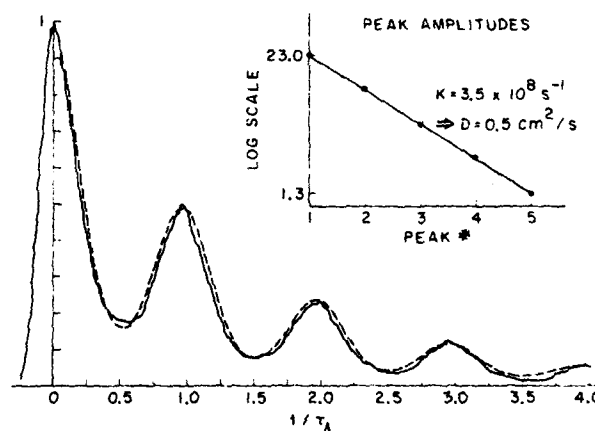
Fig. 9. Theoretical fit to second experimental plot in Fig. 3 ( \lambda = 5.3 \mu\text{m} ), for A_0 = -0.02 and A_1 = +0.37 .
