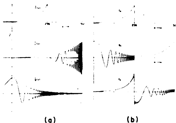
Fig. 1 (a) Exact analytical functions \hat{f}(x) , \hat{j}(x) , and \hat{g}(x) corresponding to a uniform circular "top-hat" input function f(r) and its Airy-disk Hankel transform, including the top-hat input function \hat{f} (top curve); the l = 0 Bessel-function kernel \hat{j} (middle curve); and the Airy-disk Hankel transform \hat{g} (bottom curve). Parameter values for the change of variables are \alpha = 0.01612 , r_0 = \rho_0 = 0.06349 , and \beta = b = 3.938 , corresponding to N = 256 , K_1 = K_2 = 4 . The "dimples" in the \hat{g} function at larger arguments are spurious results of a plotting routine with inadequate point spacing. (b) Discrete Hankel transformation and then backtransformation of a sampled top-hat input sequence f_n (top curve) into the transformed sequence g_n (middle curve) and then back into a sequence f_n (bottom curve), using the FHT algorithm with N = 256 , K_1 = K_2 = 4 . The portions of the transformed and backtransformed sequences g_n and f_n above n = 256 arise from aliasing effects in the transform algorithm and are discarded. The backtransformed sequence f_n exhibits Gibbs phenomena because of the finite truncation of the g_n sequence before it is backtransformed.
