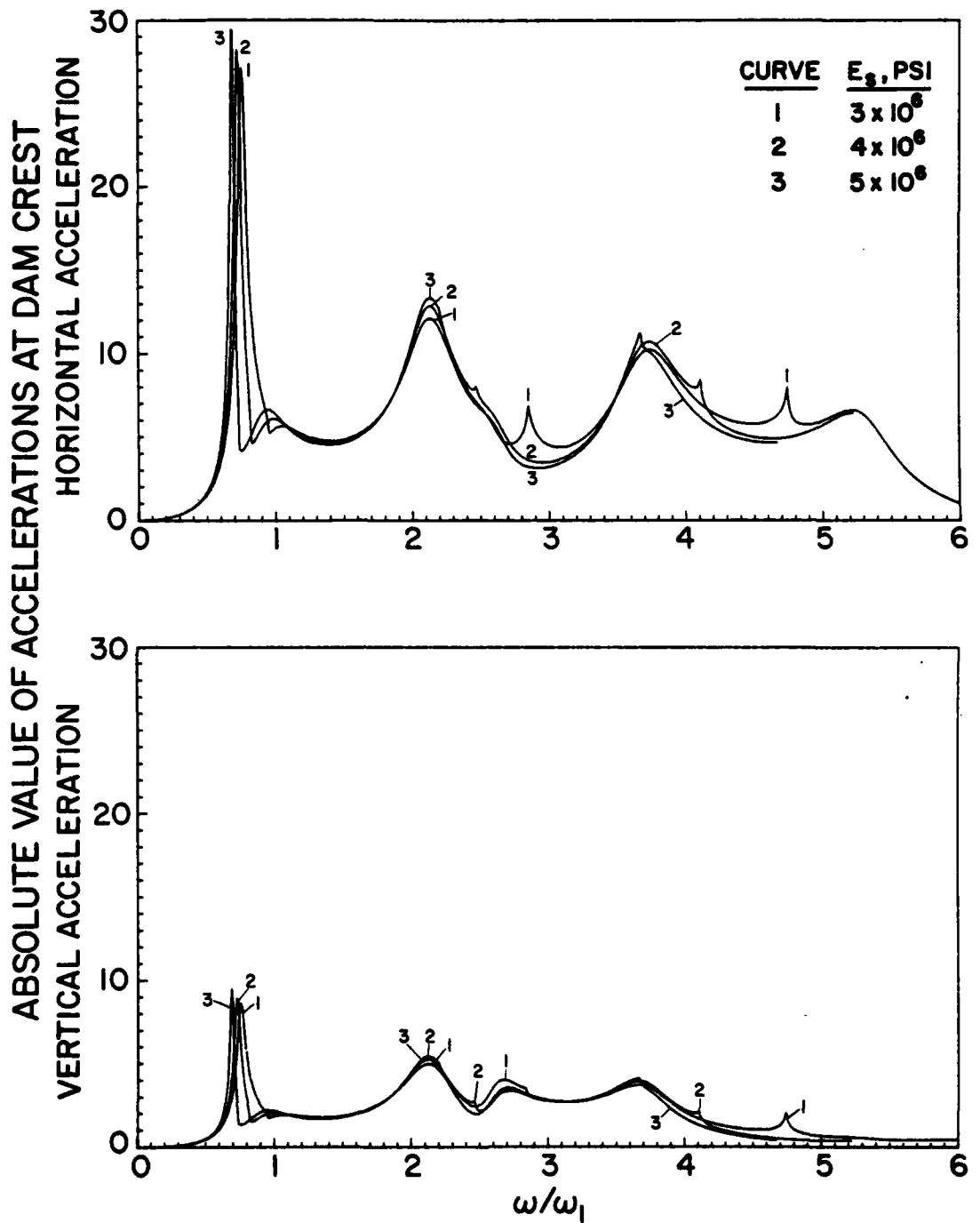
FIG. 8.4 INFLUENCE OF YOUNG'S MODULUS E_s OF DAM CONCRETE ON RESPONSE OF DAMS TO HARMONIC, HORIZONTAL GROUND MOTION. E_s IS VARIED AS SHOWN: CASES 3, 4, AND 5 OF TABLE 8.1
