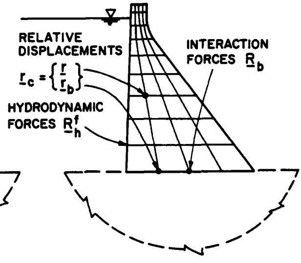
SUBSTRUCTURE 1: DAM
