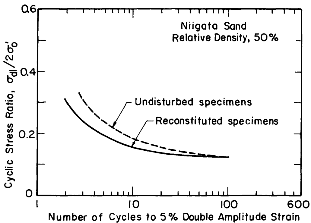
FIG. 2-6 SUMMARY CURVE COMPARING THE CYCLIC STRENGTH AT 50% RELATIVE DENSITY OF RECONSTITUTED AND UNDISTURBED SAND SPECIMENS FROM NIIGATA, JAPAN
