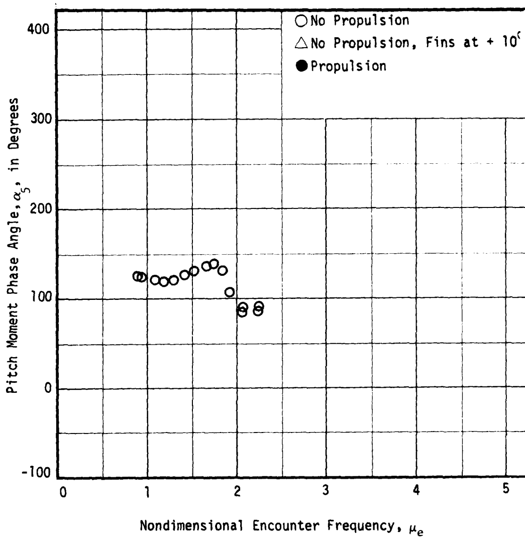
Figure 59 - Variation of Pitch Moment Phase Angle, \alpha_5 , with Nondimensional Encounter Frequency, \mu_e , at a Full Scale Speed of 4 Knots for the SWATH 60 in Following Waves
