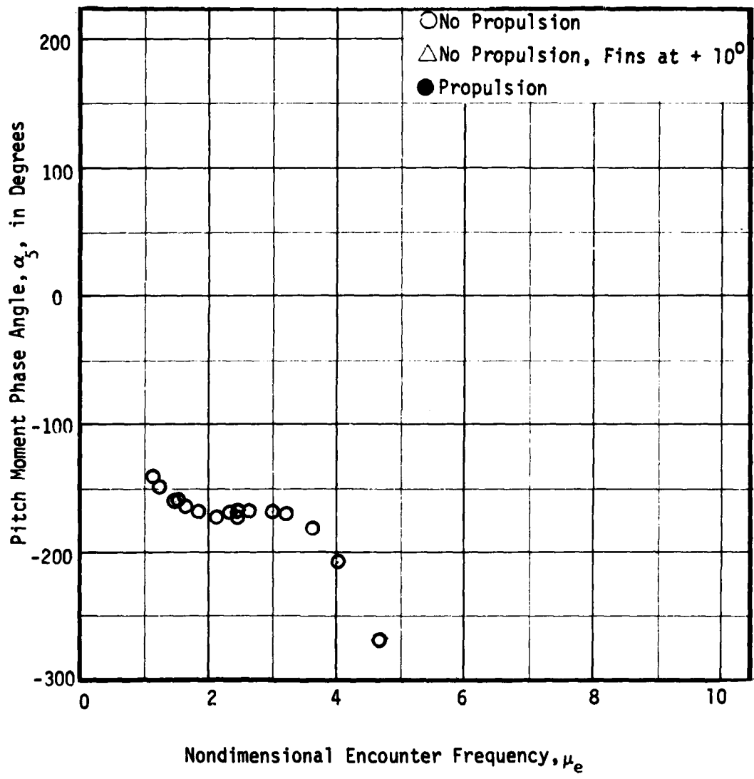
Figure 90 - Variation of Pitch Moment Phase Angle, \alpha_5 , with Nondimensional Encounter Frequency, \mu_e , at a Full Scale Speed of 7 Knots for the SSP in Head Waves
