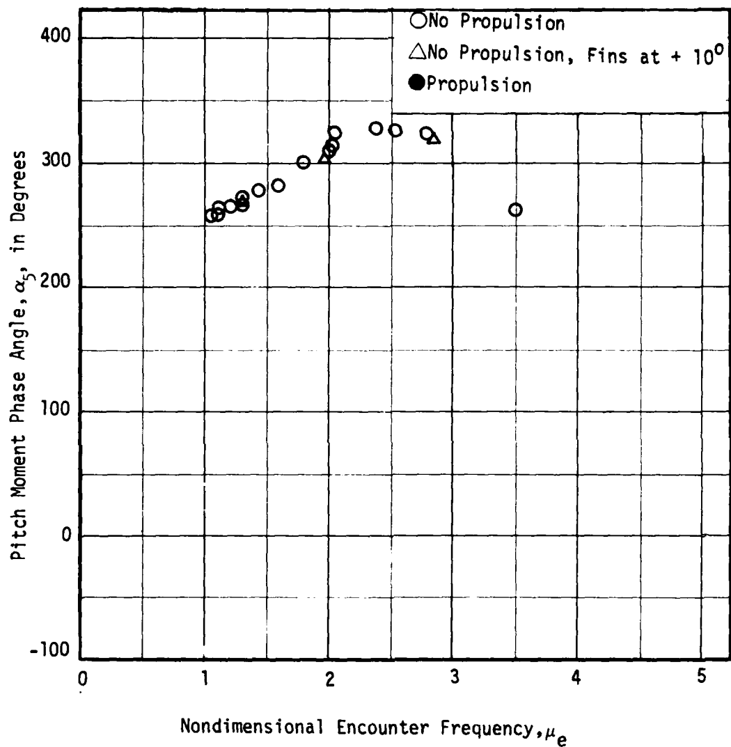
Figure 29 - Variation of Pitch Moment Phase Angle, \alpha_5 , with Nondimensional Encounter Frequency, \mu_e , at a Full Scale Speed of 4 Knots for the SWATH 6D in Head Waves
