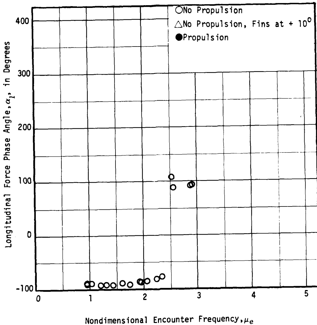
Figure 38 - Variation of Longitudinal Force Phase Angle, \alpha_1 , with Nondimensional Encounter Frequency, \mu_e , at Zero Speed for the SWATH 6D in Following Waves
