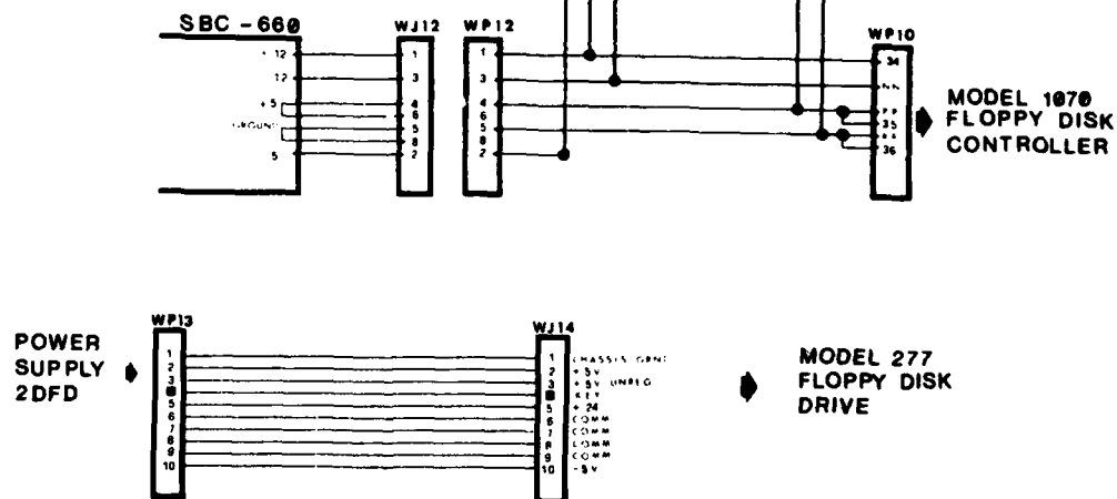
Figure 5. Floppy-disk/meter circuit.
