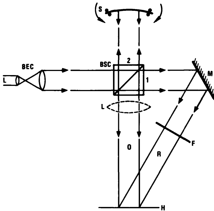
Figure A4 Laser/Optical Configuration for Measurement of Poisson's Ratio of Compliant Materials
