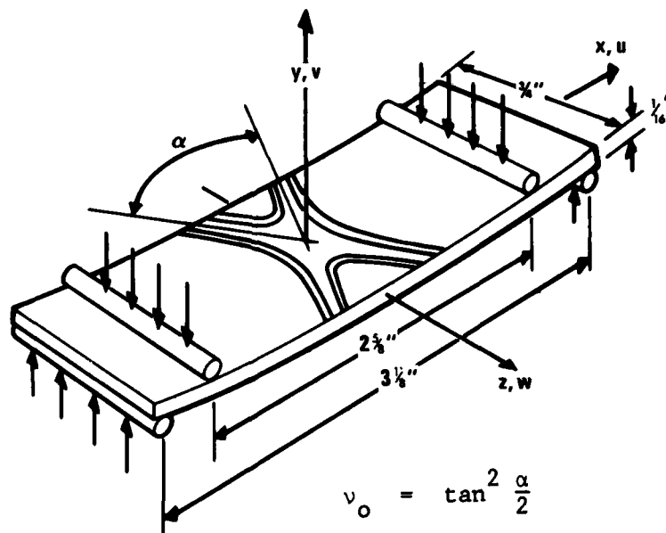
Figure A5 Test Geometry and Reference Frame
