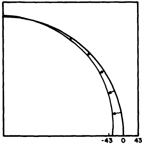
g) Normal stresses (ksi) elapsed time: 280 hours
