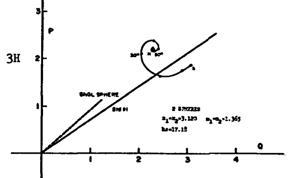
Figs. 3D-3I Same as Figs. 3A-3C.
