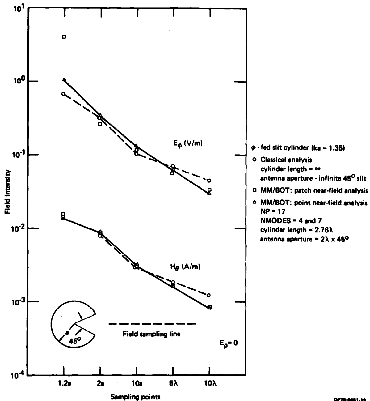
Figure 19. Computation of near fields for slit cylinder at \phi = 0 (slit angle = 45^\circ )
