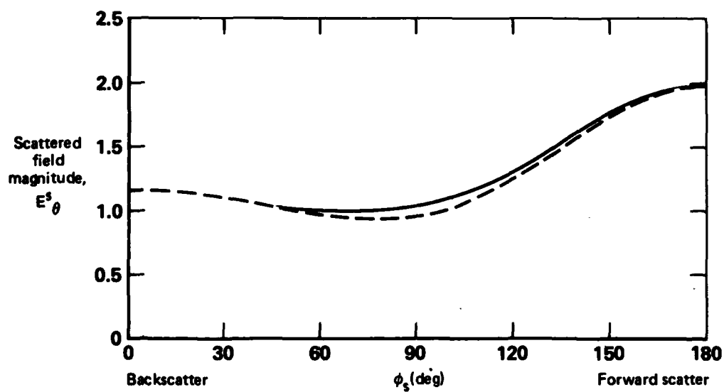
Figure 15. Bistatic scattering calculations for a square cylinder.
