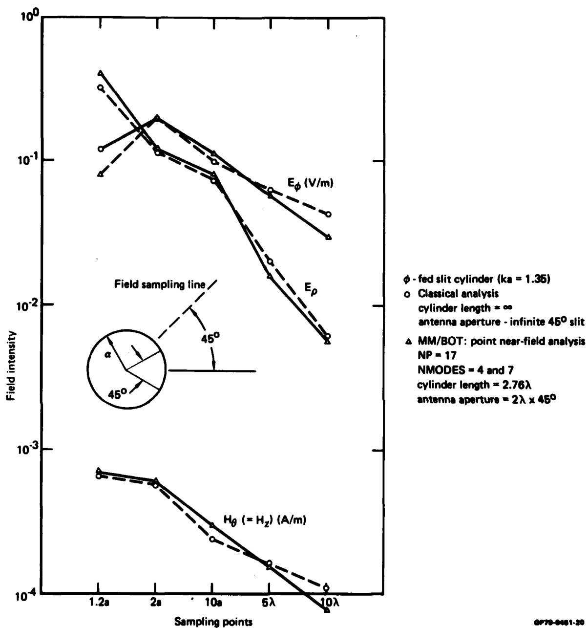
Figure 20. Computation of near fields for slit cylinder at \phi = 45^\circ (slit angle = 45^\circ )
