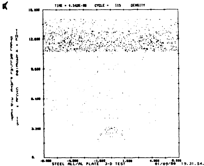
Figure A-8 Material Density Plot at Time = 4.5 \mu s K = 1 Plane Only
