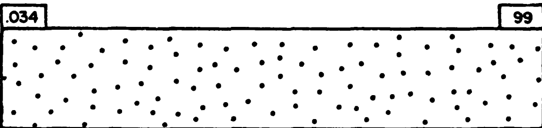
Figure 8-8. Classes 1 and 2 Weld Radiographic Inspection Standards for Randomly Dispersed Porosity (Sheet 6 of 7).
