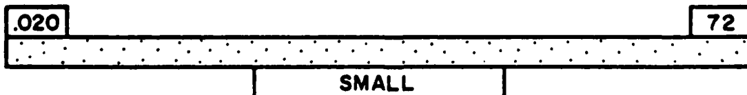
Figure 8-9. Class 3 Weld Radiographic Inspection Standards for Randomly Dispersed Porosity (Sheet 1 of 7).
