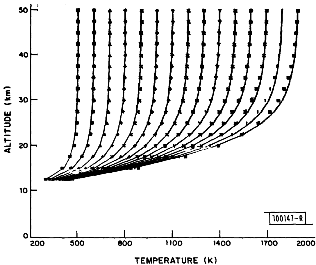
Fig. 1. CIRA temperature profiles (solid lines) and the fits afforded by Equation 6 (symbols).
