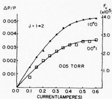
FIG. 3. Excitation of the 10^0 and 00^1 vibrational states of HCN.
