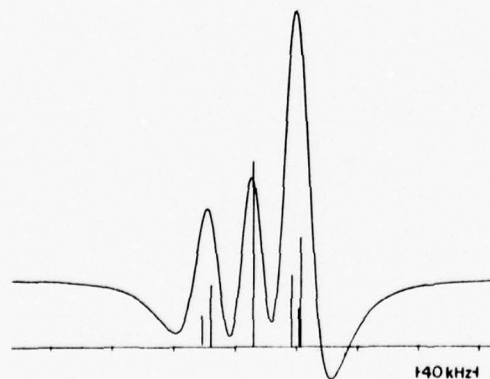
FIG. 5. Experimental and theoretical spectra of the J = 1 \rightarrow 0 , F_N = 1 transition in ND 3 .
