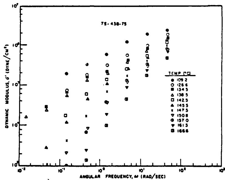
Figure 3. Dynamic Modulus as a Function of Angular Frequency.
