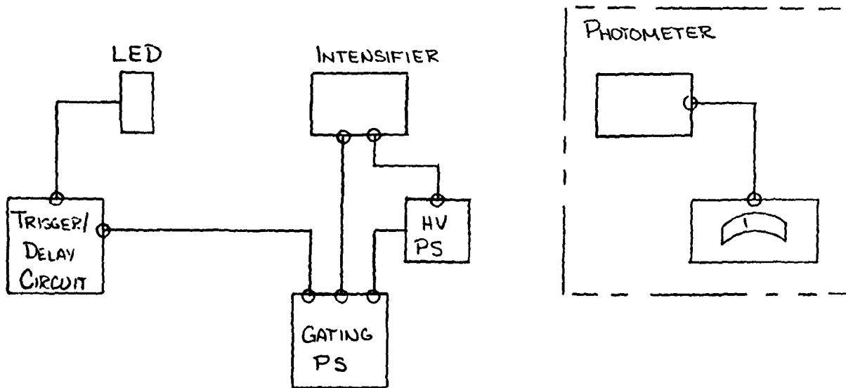
MEASUREMENT SET-UP
