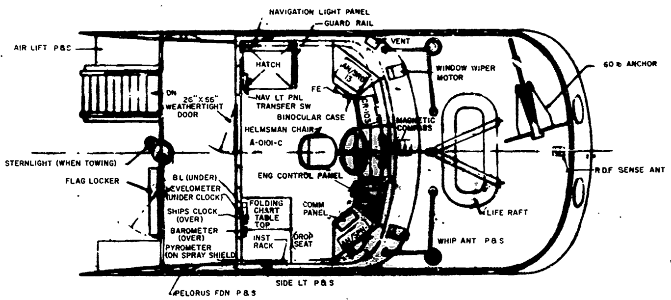
WHEELHOUSE AND CABIN TOP
