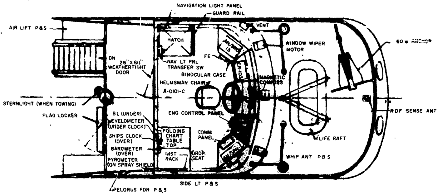
WHEELHOUSE AND CABIN TOP
