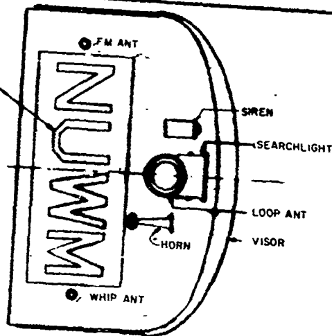
WHEELHOUSE TOP
