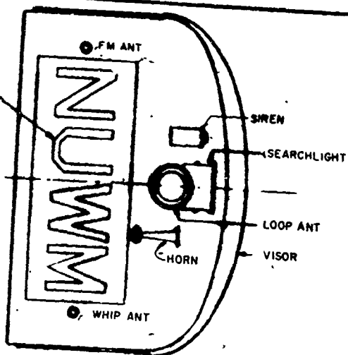
WHEELHOUSE TOP
