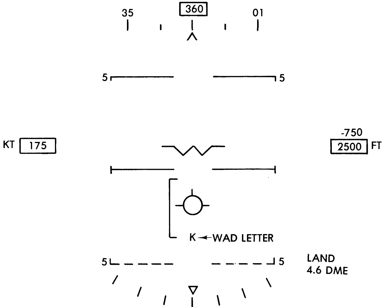
Figure 2 F/A-18 Based HUD Format
