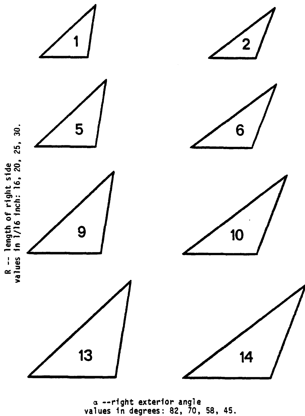
Figure 14. Experiment IV: triangles in R by \alpha set.
