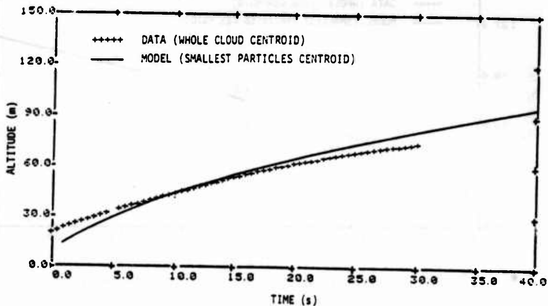
Figure 11. Dust cloud centroid altitude for event B6.
