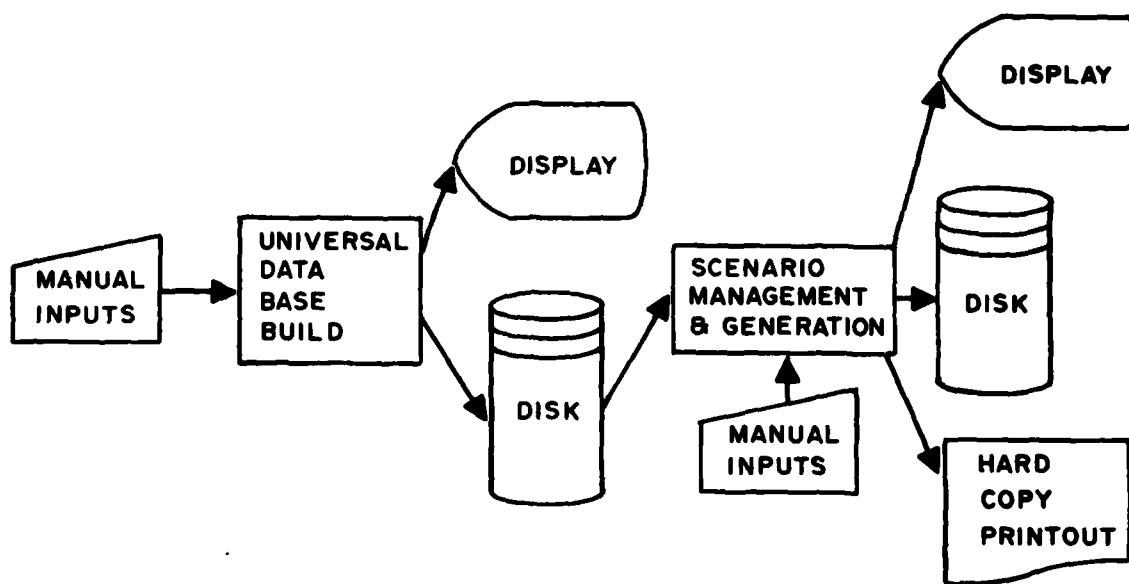
FIGURE 3. Scenario generation.
