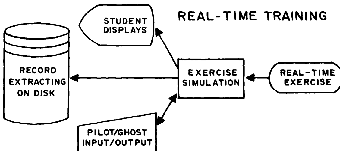
FIGURE 4. Real-time training.
