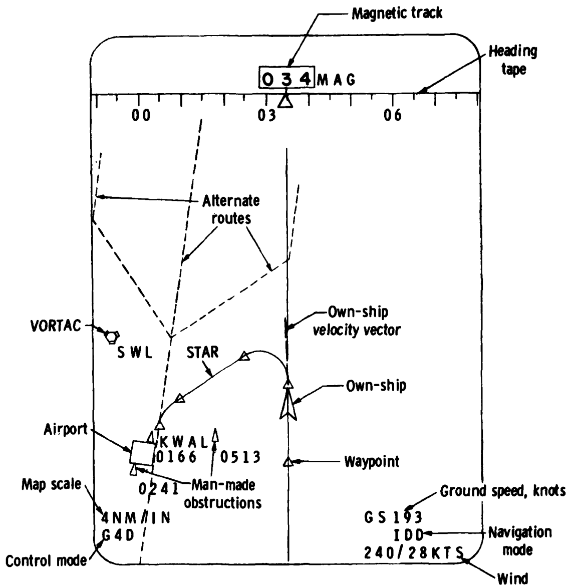
Figure 5.- Electronic situation indicator format. (1 inch = 2.54 cm.)
