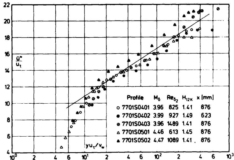
Fig. 4.4.14 Law of the wall for a compressible boundary layer (adiabatic wall, zero pressure gradient, defined origin). Mabey (1977).
