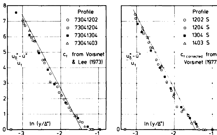
Fig. 5.2.8 Outer law for a compressible boundary layer in a favourable pressure gradient (isothermal wall, origin not defined) Voisinnet & Lee (1973).
