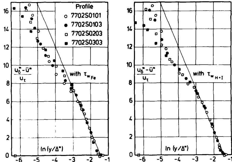
Fig. 4.3.4 Outer law for a compressible turbulent boundary layer (adiabatic wall, zero pressure gradient, defined origin). Ladernan & Demetriades (1977).
