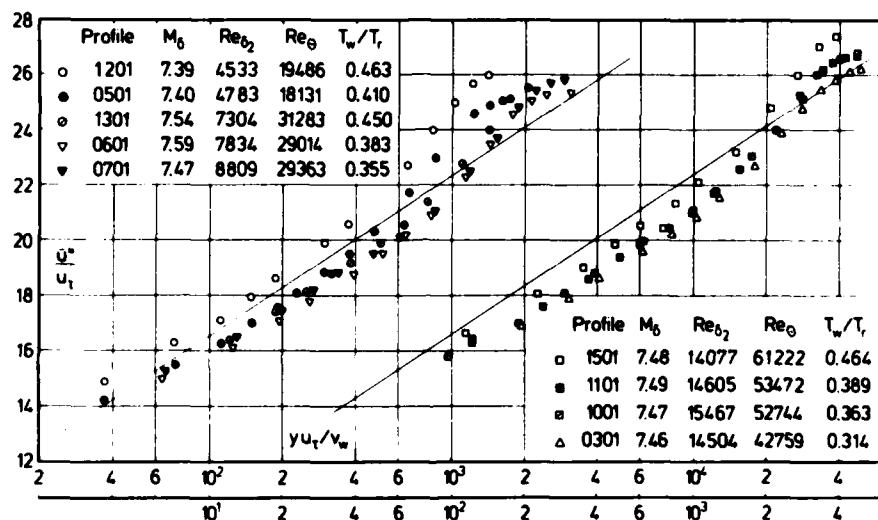
Fig. 4.3.7 Law of the wall for a compressible boundary layer (isothermal wall, zero pressure gradient, no defined origin). Hopkins & Keener (1972).
