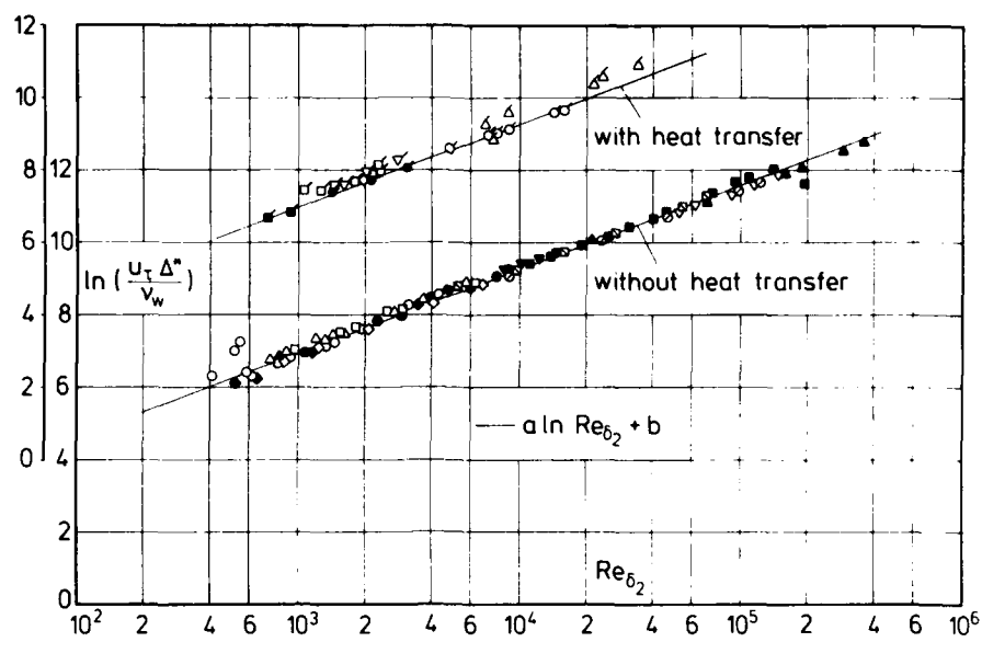
Fig. 3.3.5 Relationship between the characteristic Reynolds numbers u_{\tau} \Delta^* / \nu_w and u_{\delta} \rho_{\delta} \delta_2 / \mu_w for compressible turbulent boundary layers (isothermal and adiabatic walls, zero pressure gradient)
