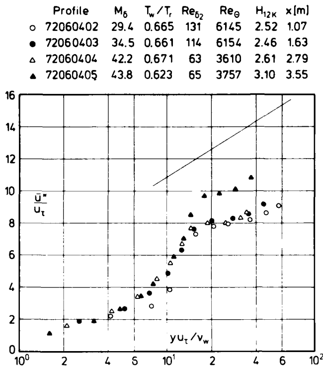
Fig. 5.2.17 Law of the wall for a compressible boundary layer with a favourable pressure gradient along an isothermal wall. Kemp & Owen (1972). c_f from FEB.
