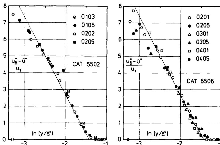
Fig. 4.6.5 Outer law for compressible turbulent boundary layers along rough walls (adiabatic and isothermal wall, zero pressure gradient, defined origin). Shutts & Fenter (1955); Young (1965).
