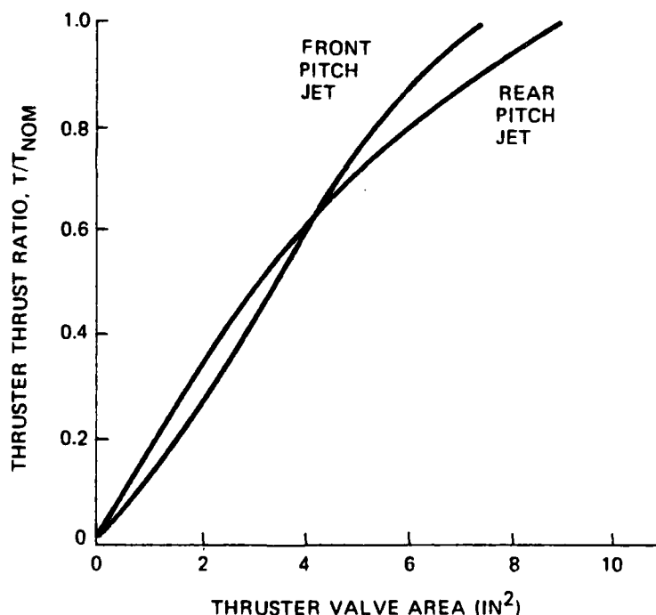
Figure C-9 Pitch Jet Thrust Ratio vs Jet Area
