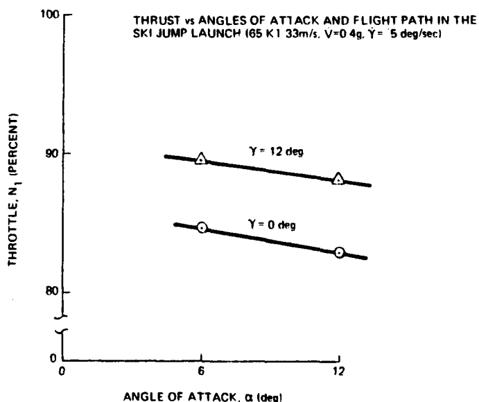
Figure 21 Thrust vs Angles of Attack and Flight Path in the Ski-Jump Launch
