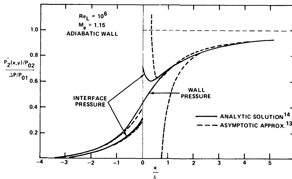
Figure 20 Comparison of Results Obtained by Analytical Solution and Asymptotic Approximation
