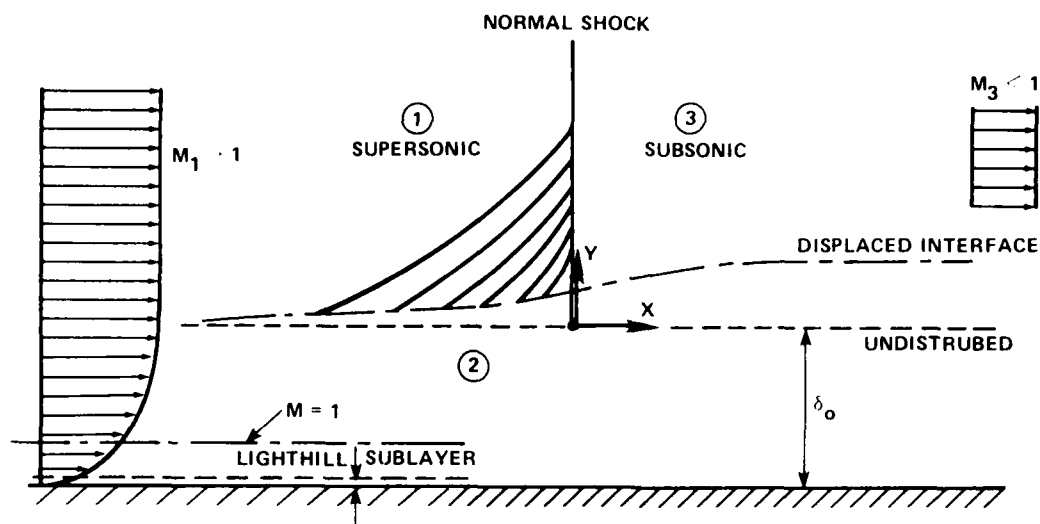
Figure 19 Schematic of Flow Model for Analytical Investigation of Transonic Viscous-Inviscid Flow Used by Manson and Inger
