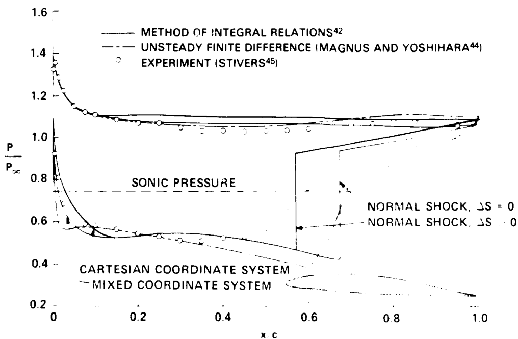
Figure 5 Pressure Distribution on an NACA 64A410 Airfoil at M_\infty = 0.72 and \alpha = 4^\circ
