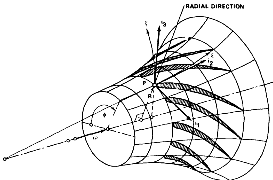
Figure 31 – Quasi Two-Dimensional Flow on Axisymmetric Stream Surface (Illustration based on Ref. 85)
