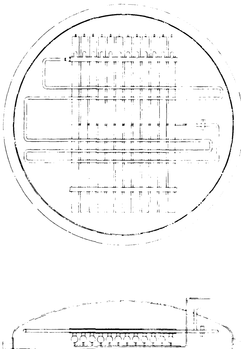
Fig. 14 — Boiler-superheater as redesigned for 2 MWhr tank. Twelve boiler tubes are used in parallel. The parallel superheater lines shown in Fig. 13 have been replaced by a single superheater line of similar total length. Series flow design provides better heat transfer to the moving steam.
