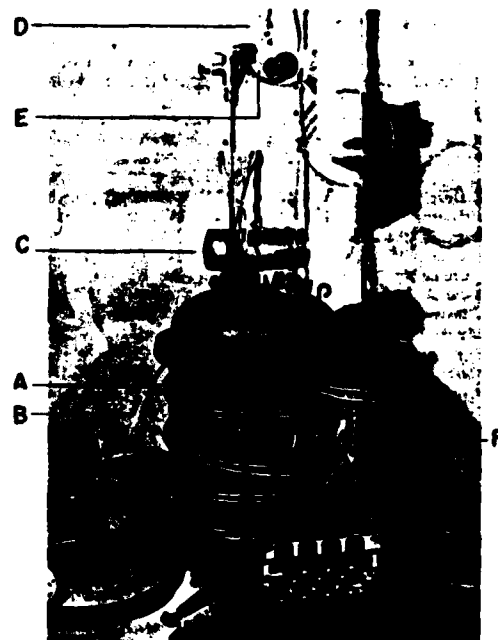
Fig. 1. A, Laboratory test tank; B, metal O-Ring used to seal domed lid to tank body; C, buffer tank; D, heated vent line; E, heated vent valve; F, thermocouple.
