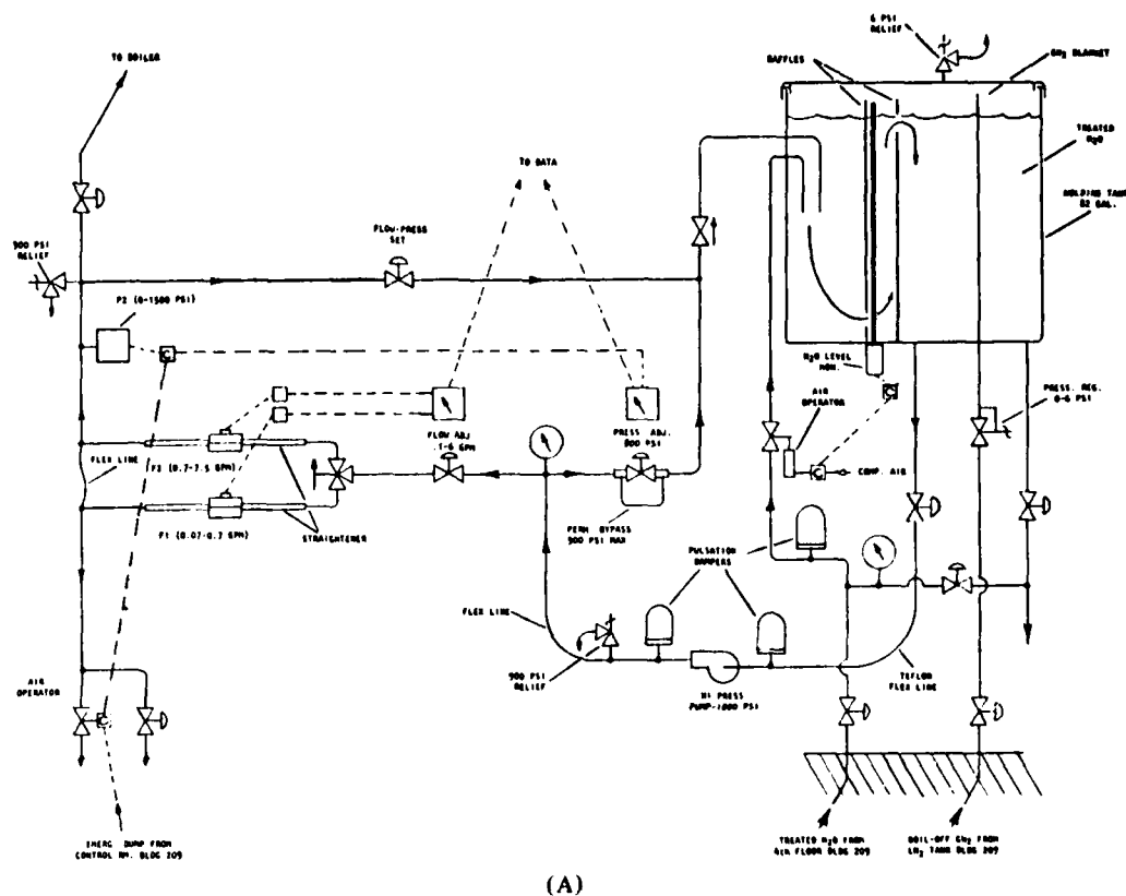
Fig. 19 — Water-steam system. Fig. 19A shows the complete loop. Fig. 19B shows an enlarged view of the low pressure water supply portion of Fig. 19A. Fig. 19C shows an enlarged view of the high pressure portion of Fig. 19A. Referring to Fig. 19B, at the bottom left of the figure, treated water is received at the site from an underground water line originating at a nearby NRL building. This water flows into a nitrogen-blanketed on-site holding tank in which the water level is controlled in response to a level control. A pulsation damper is included in the input line to reduce pressure surges which could otherwise damage the underground feed line when flow is cut off. Stored water is fed to the high pressure feedwater pump under gravity head by means of a teflon flex line, which exits Fig. 19B near the left bottom of the figure. Referring to Fig. 19C, low pressure water enters the figure at the bottom right, going directly to the high pressure feedwater pump. The main flow proceeds to a T, at which a pressure gauge is shown. It turns left at the T and passes through a selectable flow meter to the feedwater header at the left edge of the figure. It then proceeds up the figure to the boiler. The high pressure feedwater system also contains two bypass loops in parallel with the boiler. The first of these bypasses, which is the only one used during actual boiler operation, is an adjustable by-pass by which high pressure water flow is dropped to low pressure and returned to the on-site holding tank shown in Fig. 19B. When only a small amount of steam is being withdrawn from the energy storage tank, most of the high pressure water flow passes through the adjustable by-pass. This permits the feedwater pump to operate at its normal pumping speed. The second by-pass is the horizontal line at the top of Fig. 19C. It is used by the operator to set up desired water flow conditions prior to passing water into the boiler. When steam generation is desired, the valve (top left) to the boiler is opened and the upper by-pass is closed off.
