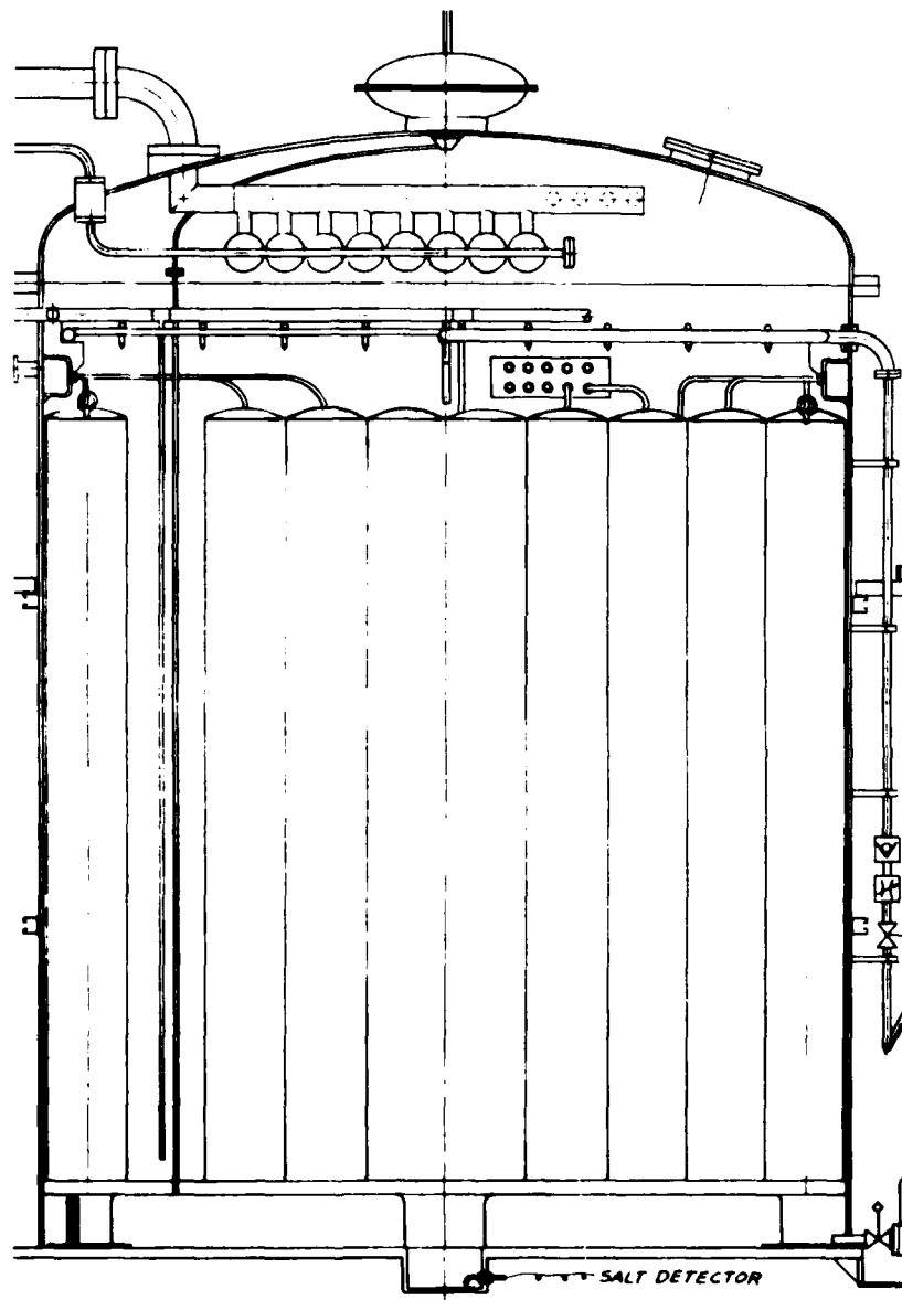
Fig. 6 — Energy storage boiler tank with separately manifolded salt cans. Because \text{MgCl}_2 , \text{NaCl} , \text{KCl} salt eutectic freezes into a porous block in the presence of terphenyl vapor, it may be desirable to provide an inert atmosphere in contact with the salt. Such an atmosphere can be provided in a practical manner by using very large salt cans which are individually manifolded to an inert gas supply whose pressure is made to follow the terphenyl pressure within the tank. The figure shows large verticle salt cans filling the bulk of the tank, terphenyl shower heads above the salt cans, and the condensation boiler inside the tank dome. The rectangular plate with gas ports below the shower heads, and the two rectangular boxes shown in cutaway on the left and right tank wall interiors are the inert gas manifolds from which gas is distributed to each of the salt containment cans. Gas tubes (8 shown) are connected between the inert gas manifold and a connection on each salt can. The large salt containers are 12 inches in diameter and must have internal heat conduction means to deliver heat to the salt with acceptably low temperature drop, as shown in Figure 7. This design concept is not used in the NRL tank.
