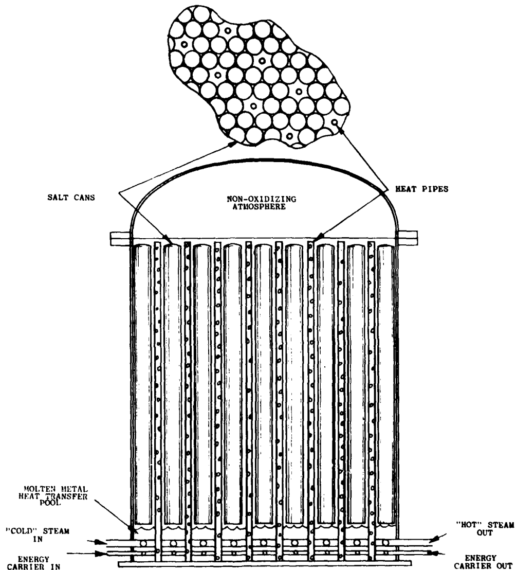
Fig E-1 — Radiation coupled energy storage tank. Operation is described in caption of Fig. 4. Salt can-heat pipe geometry on which calculations are based consists of hexagons made up of six 6-inch diameter salt cans surrounding single 2-inch diameter potassium vapor heat pipes. The configuration for a 2 MWht tank contains 53 heat pipes with an aggregate area of 2.6 \times 10^5 \text{ cm}^2 . The overall tank size is the same as that of the 2 MWht energy storage boiler tank being built at NRL, i.e., ~ 10.5' in diameter, ~ 15' high.
