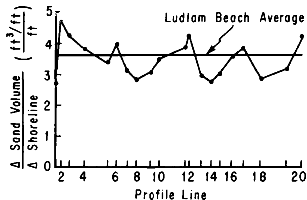
Figure 70. Mean sand volume changes above MSL which accompany shoreline retreat or advance along Ludlam Beach.
