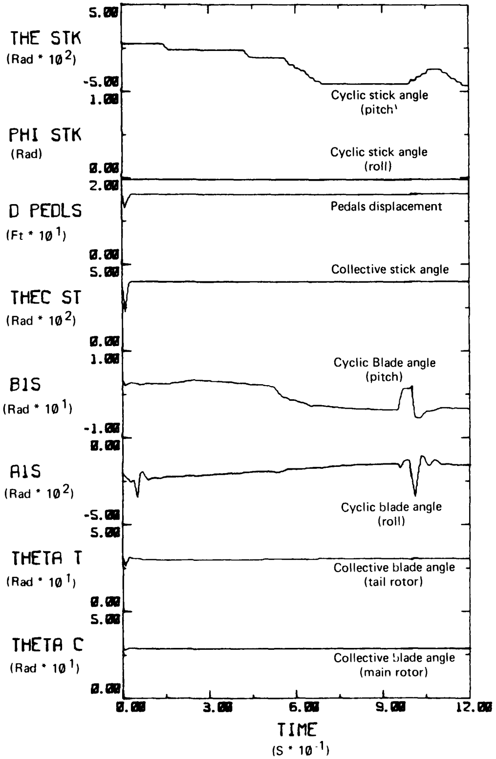
FIG 18B. SEA KING MK 50: TIME HISTORIES FOR VARIABLES (TEST 1)
