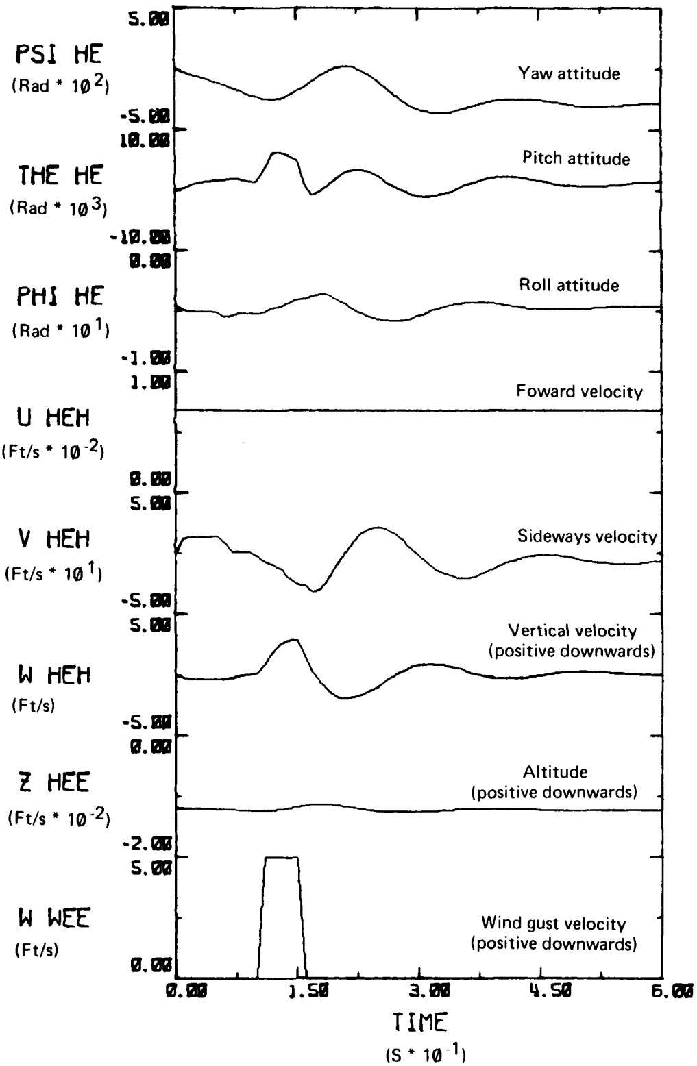
FIG 19. MODERNIZED WESSEX: TIME HISTORIES FOR VARIABLES (TEST 2)
