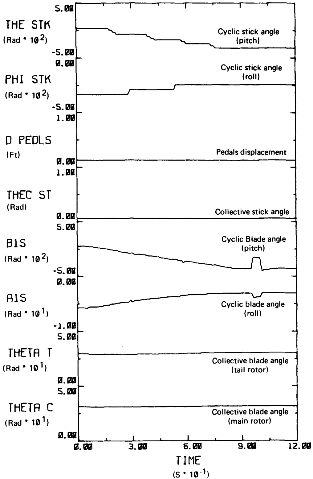
FIG 16B. MODERNIZED WESSEX: TIME HISTORIES FOR VARIABLES (TEST 1)
