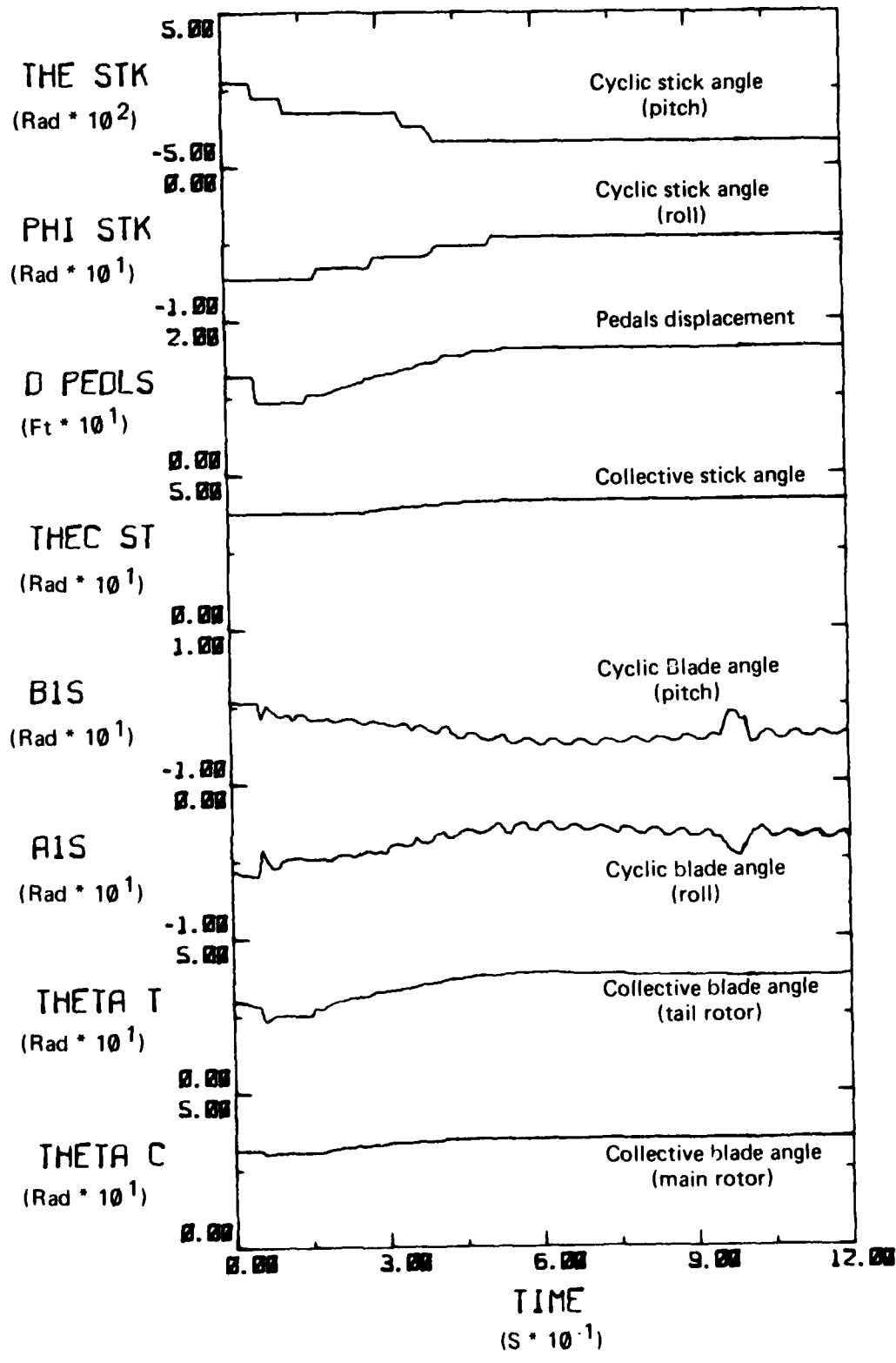
FIG 17B. WESSEX MK 31B: TIME HISTORIES FOR VARIABLES (TEST 1)
