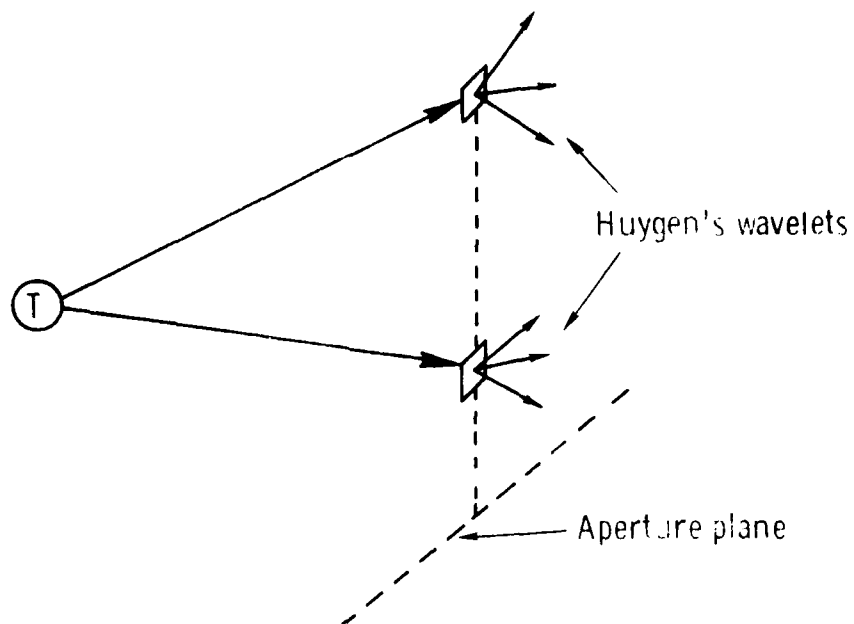
Fig.4-1. Huygen's principle.
