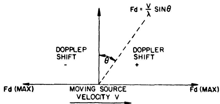
(a) THE DOPPLER PRINCIPLE
