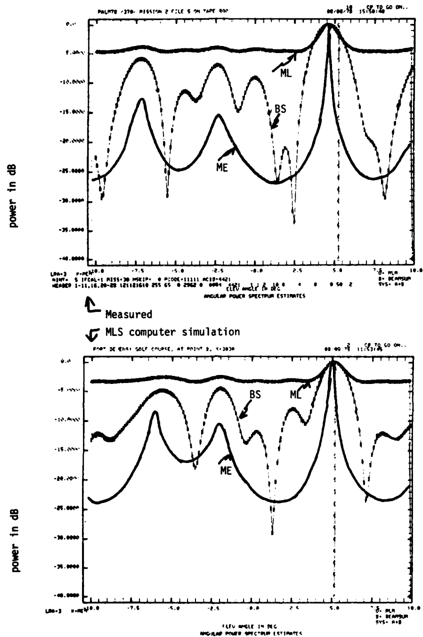
Fig. 2-32. Fort Devens measurement (golf course): \theta = 5.2^\circ .
