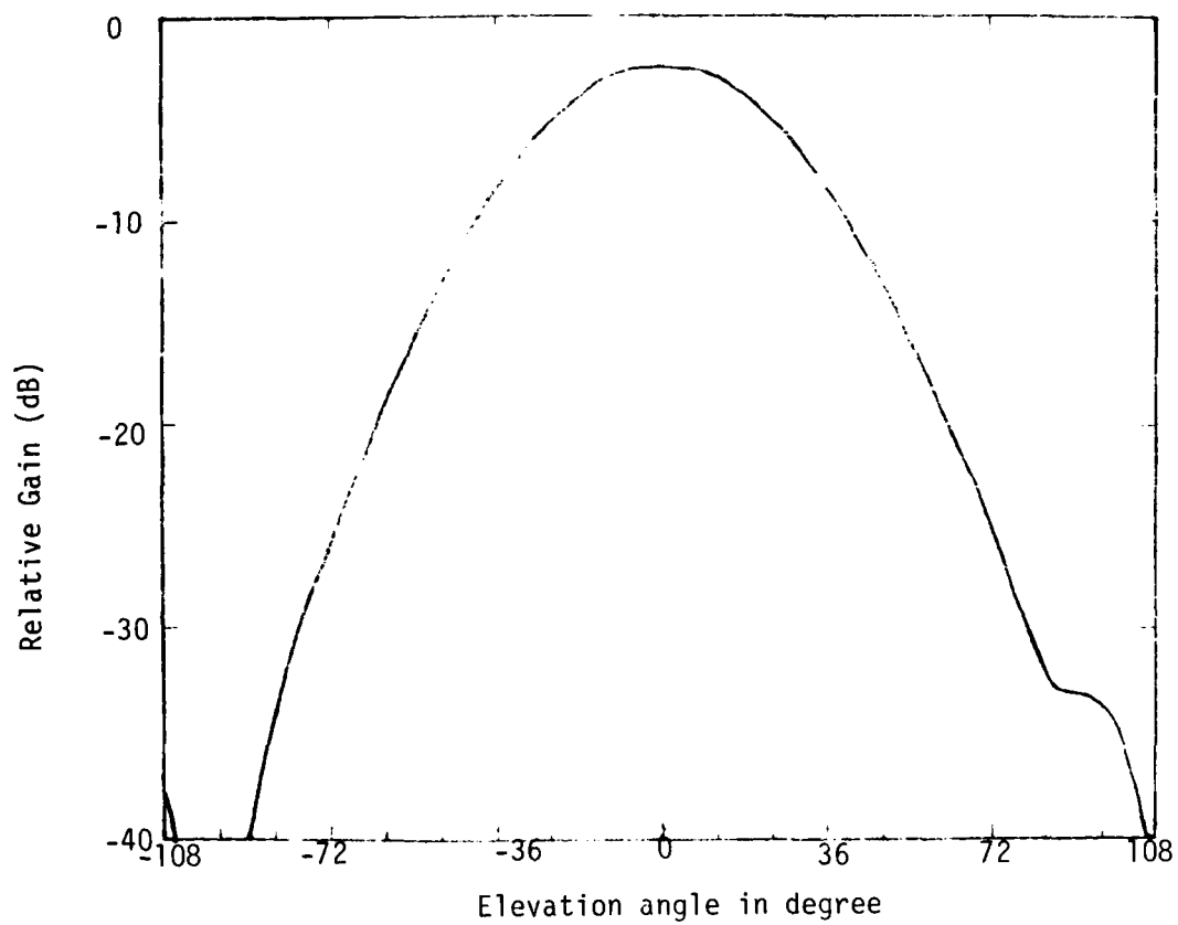
Fig.2-5. E-plane radiation pattern.
