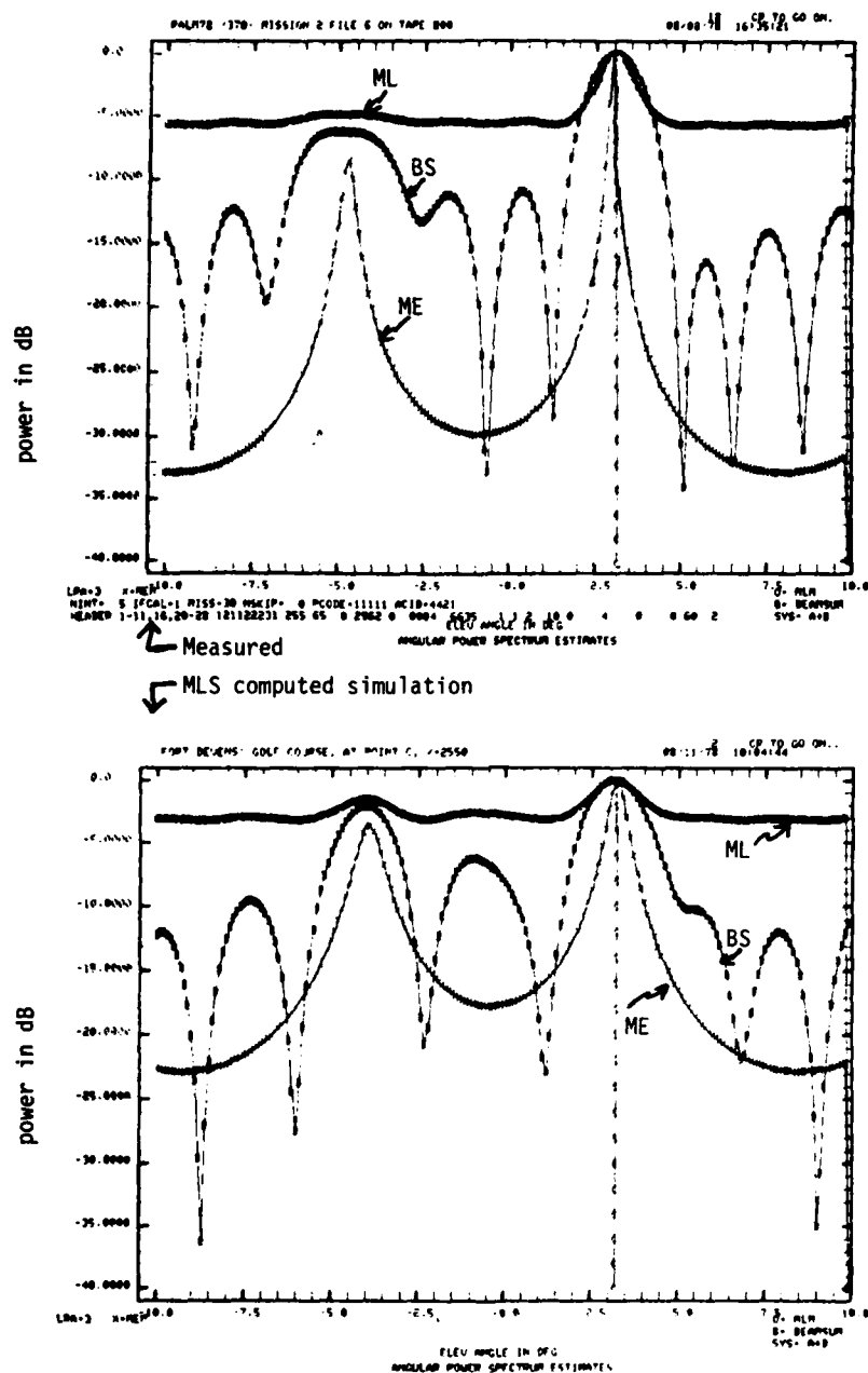
Fig. 2-28. Fort Devens measurement (golf course): \theta = 3.2^\circ .
