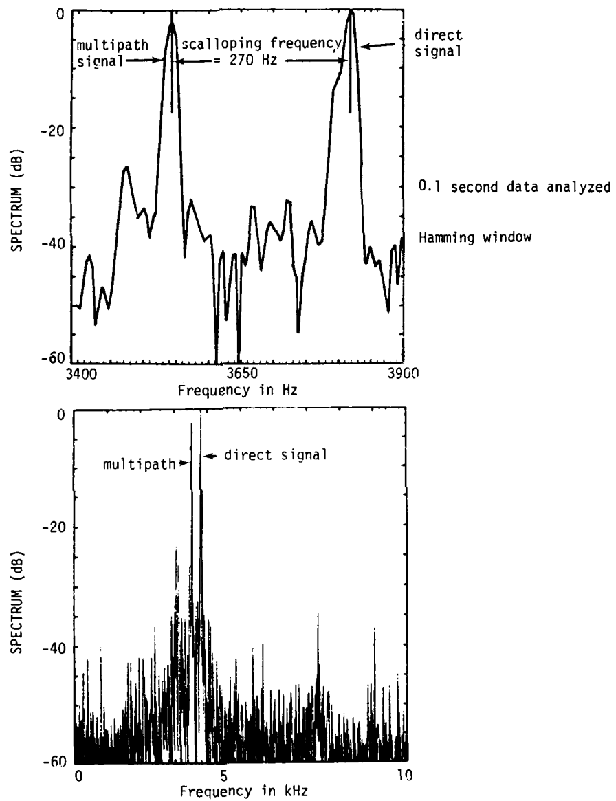
Fig.3-73. Spectrum of demodulated signal: example of WPAFB multipath at 270 Hz scalping frequency.
