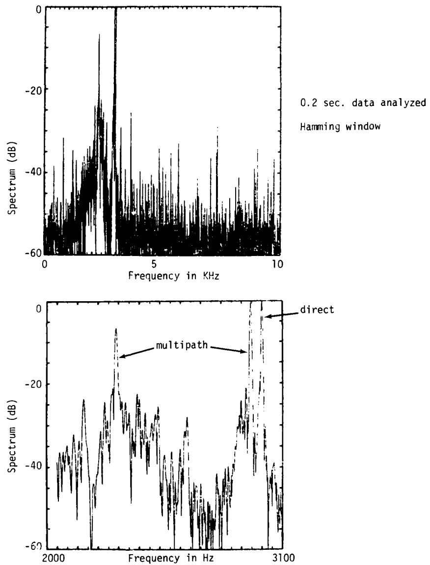
Fig.3-64. Example of Tulsa multipath spectrum containing both the 50 Hz scalloping frequencies and 2000 to 3100 Hz blow-up from run 5.
