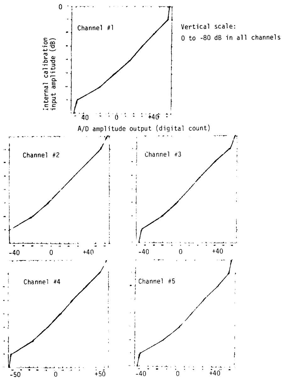
Fig.2-8. RF receiver channel amplitude output characteristics.
