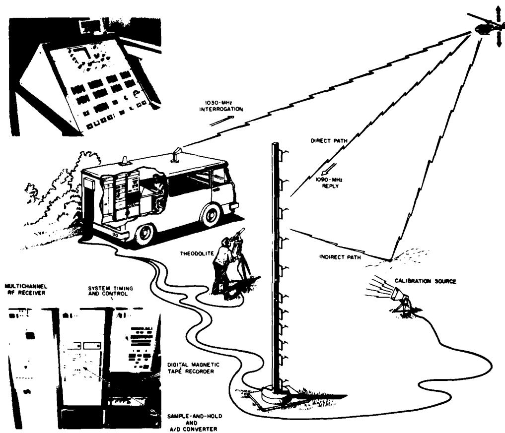
Fig.2-3. Terrain multipath experimental configuration.
