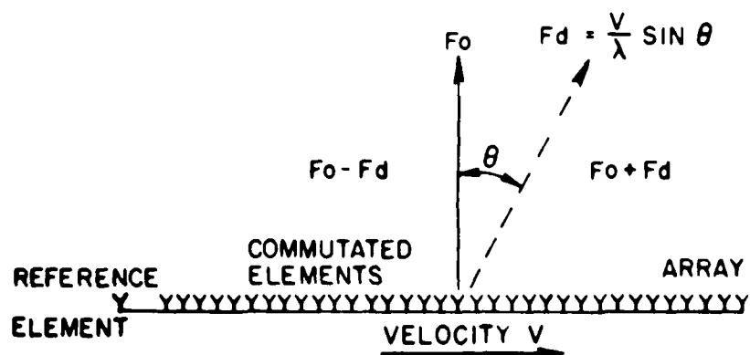
(b) DOPPLER APPLIED TO MLS
