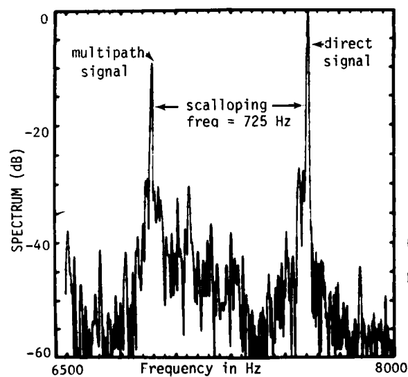
Fig.3-53. Example of St.Louis multipath near 700 Hz scalloping frequency.
