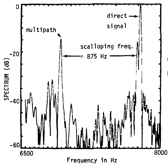
Fig.3-54. Example of St.Louis multipath near 875 Hz scalloping frequency.
