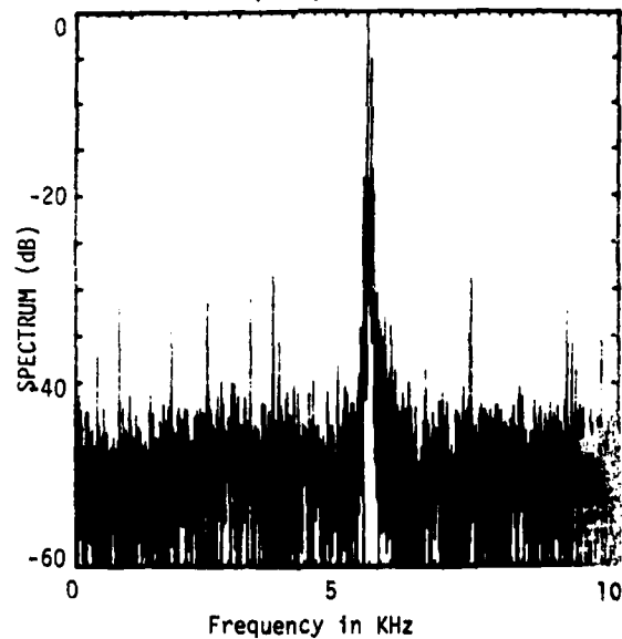
Fig. 89(b). Miami demodulated signal spectrum in high level multipath region on run #5.
