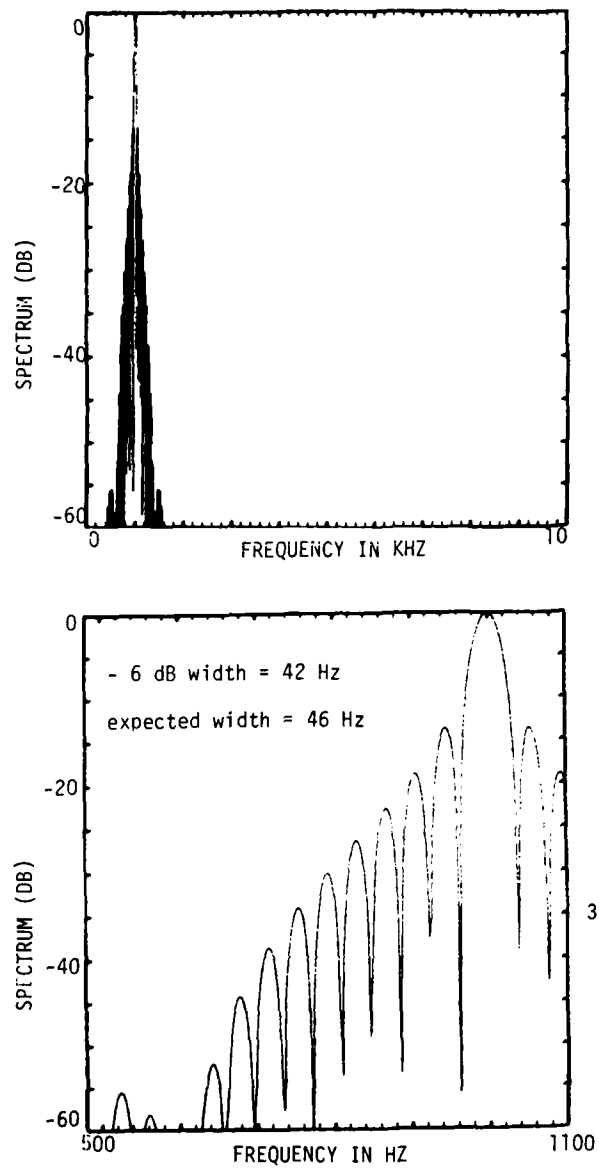
Fig.3-34. Tukey 25% window applied to synthetic data.
