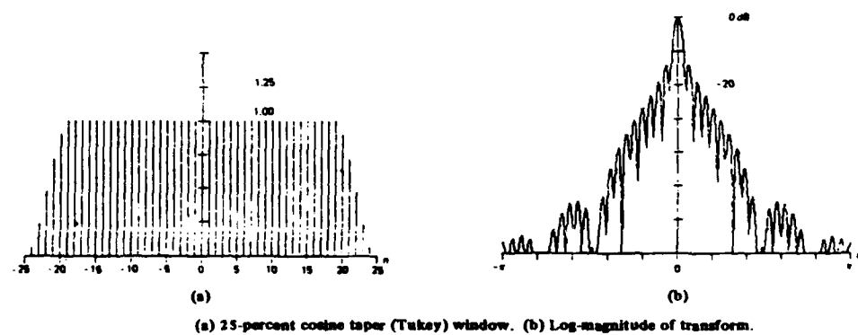
Fig.3-32. Spectrum analysis windows used in data reduction (from [54]).
