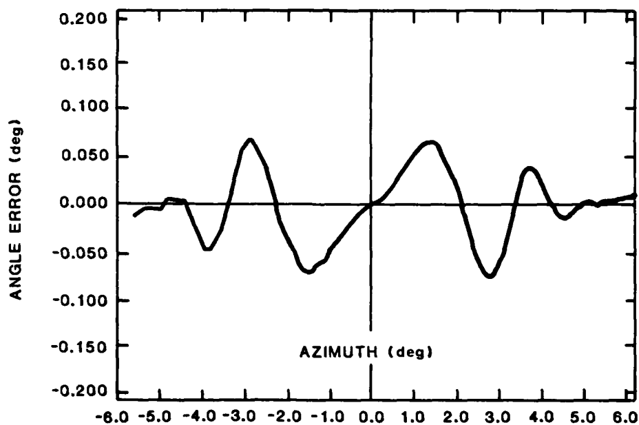
Fig.4-17. Comparison of field data and refined model.
