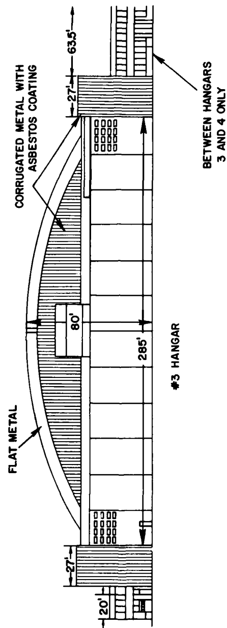
Fig. 3-3. Runway facing profile of hangar 3 at JFK.
