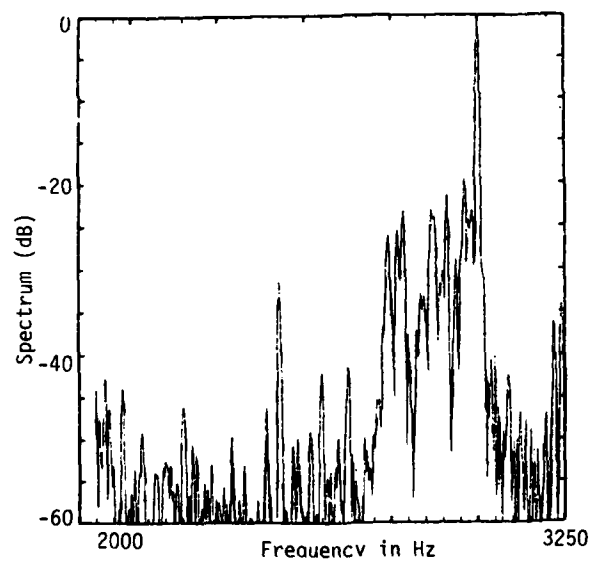
Fig.3-63. Spectrum of demodulated signal at Tulsa and a blow-up of the 1900 to 3250 Hz section from run 5.
