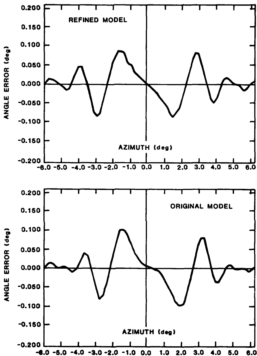
Fig.4-20. Comparison of original and refined shadowing models for Bendix small community azimuth shadowing geometry.
