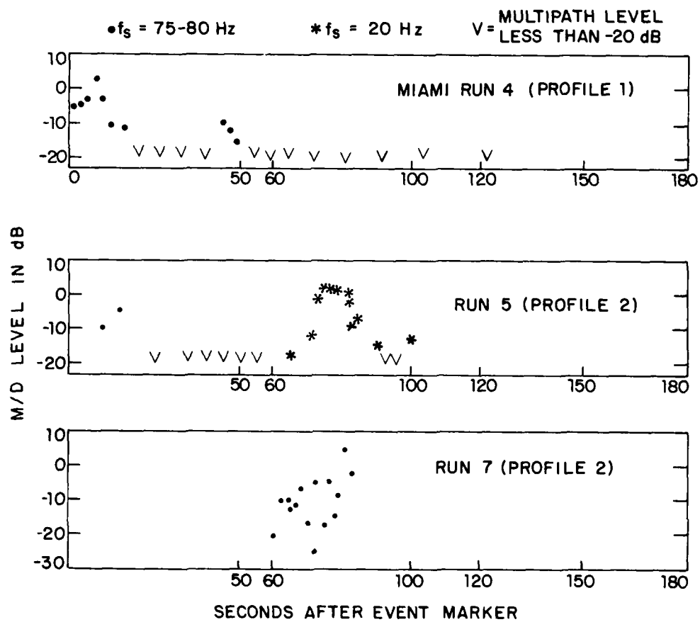
Fig. 3-92. Spectrum analysis results for Miami measurements.
