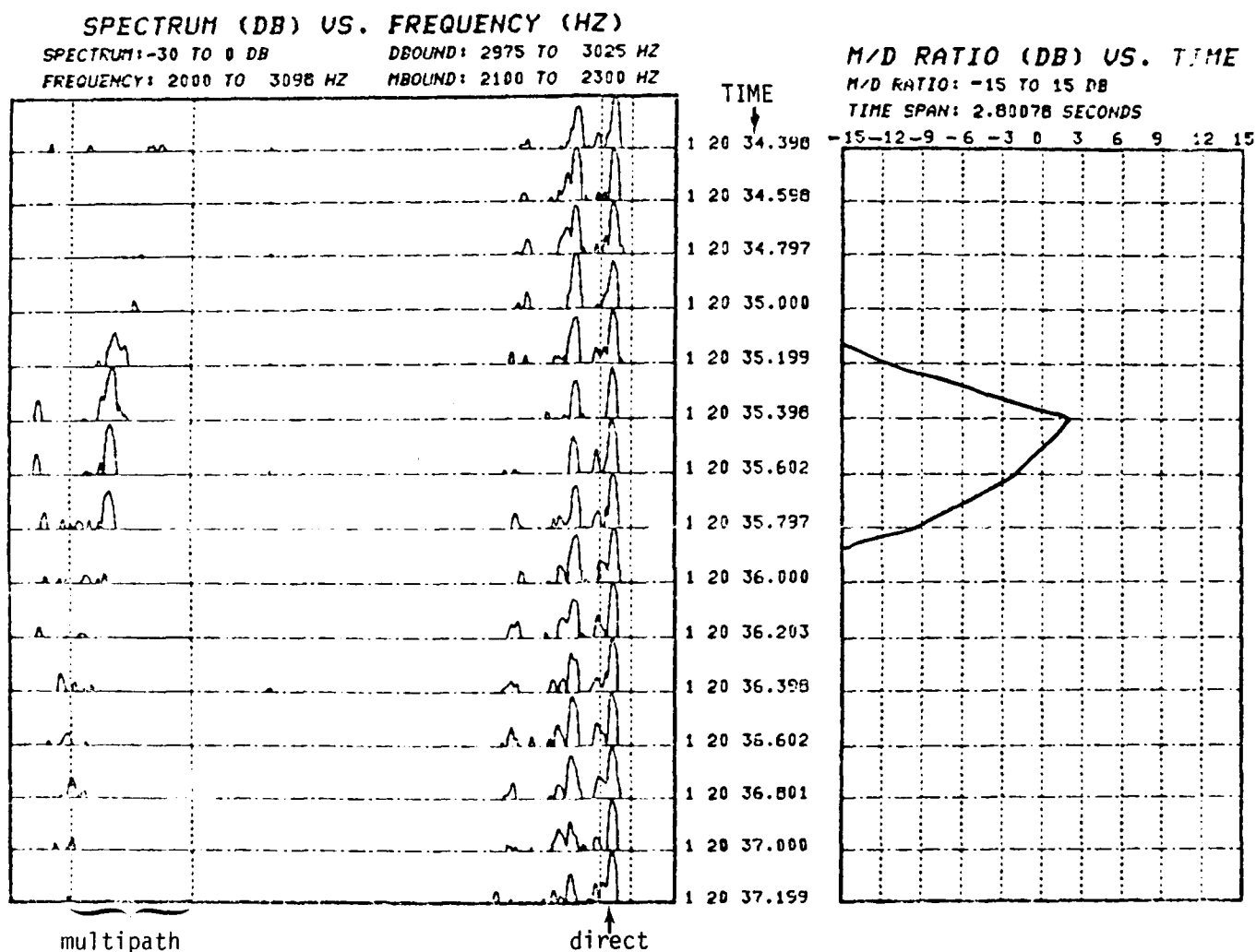
Fig.3-66. Blow-up of sequence of spectra for Tulsa run 5 from 1/20/34.298 to 1/20/37.199.
