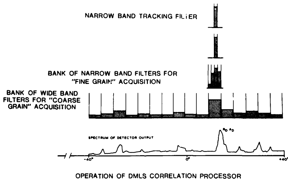
Fig.1-7. Angle estimation by DMLS receiver.
