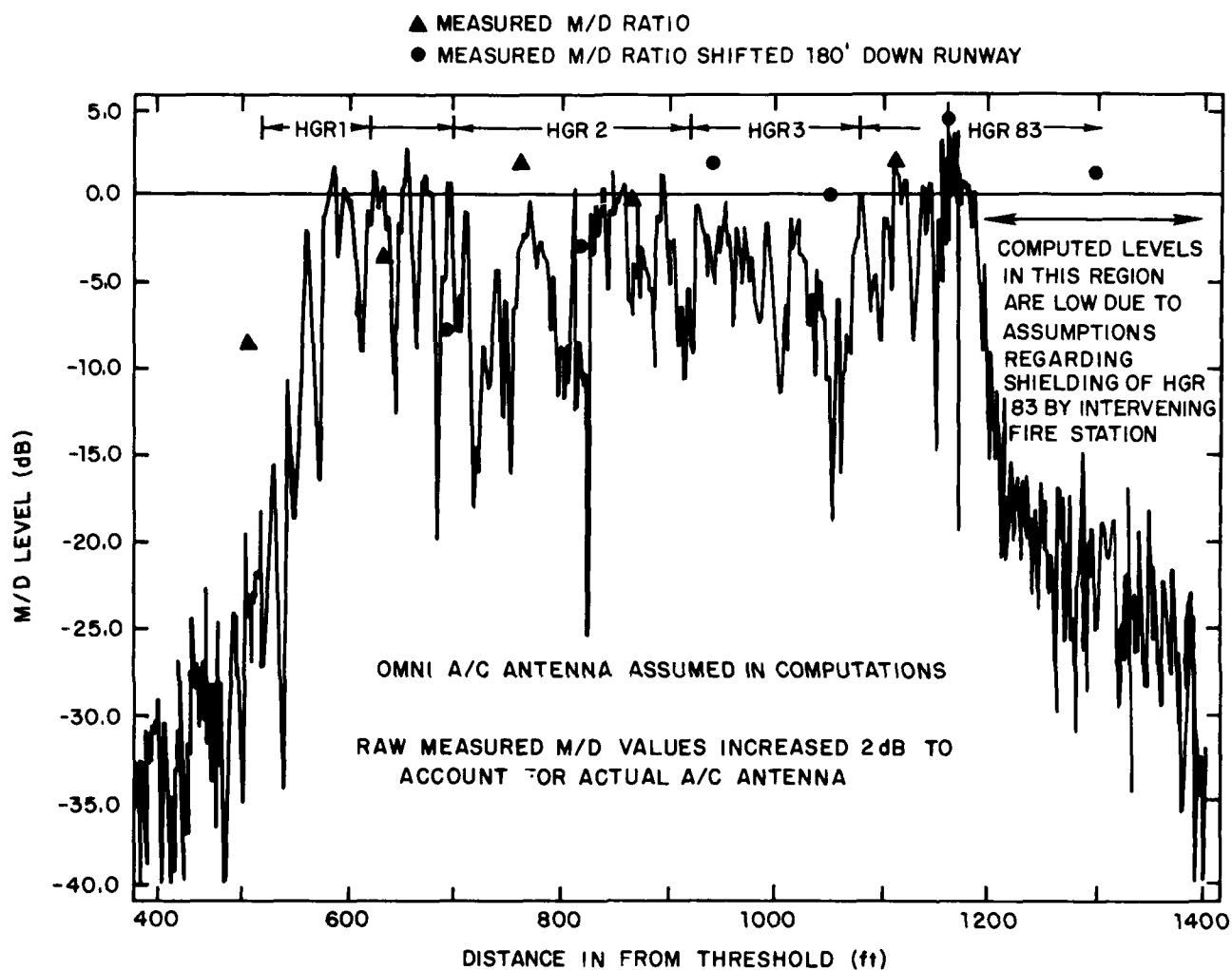
Fig. 3-105(a). Simulation results for received M/D levels.
