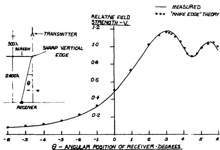
Fig. 4-23. Knife edge diffraction (from Oreb [80]).
