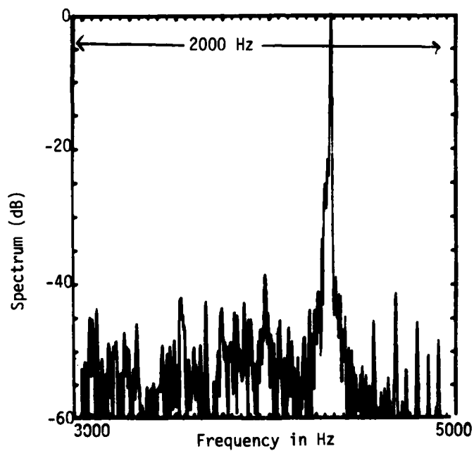
Fig. 3-51. Spectrum of demodulated signal at St. Louis.
