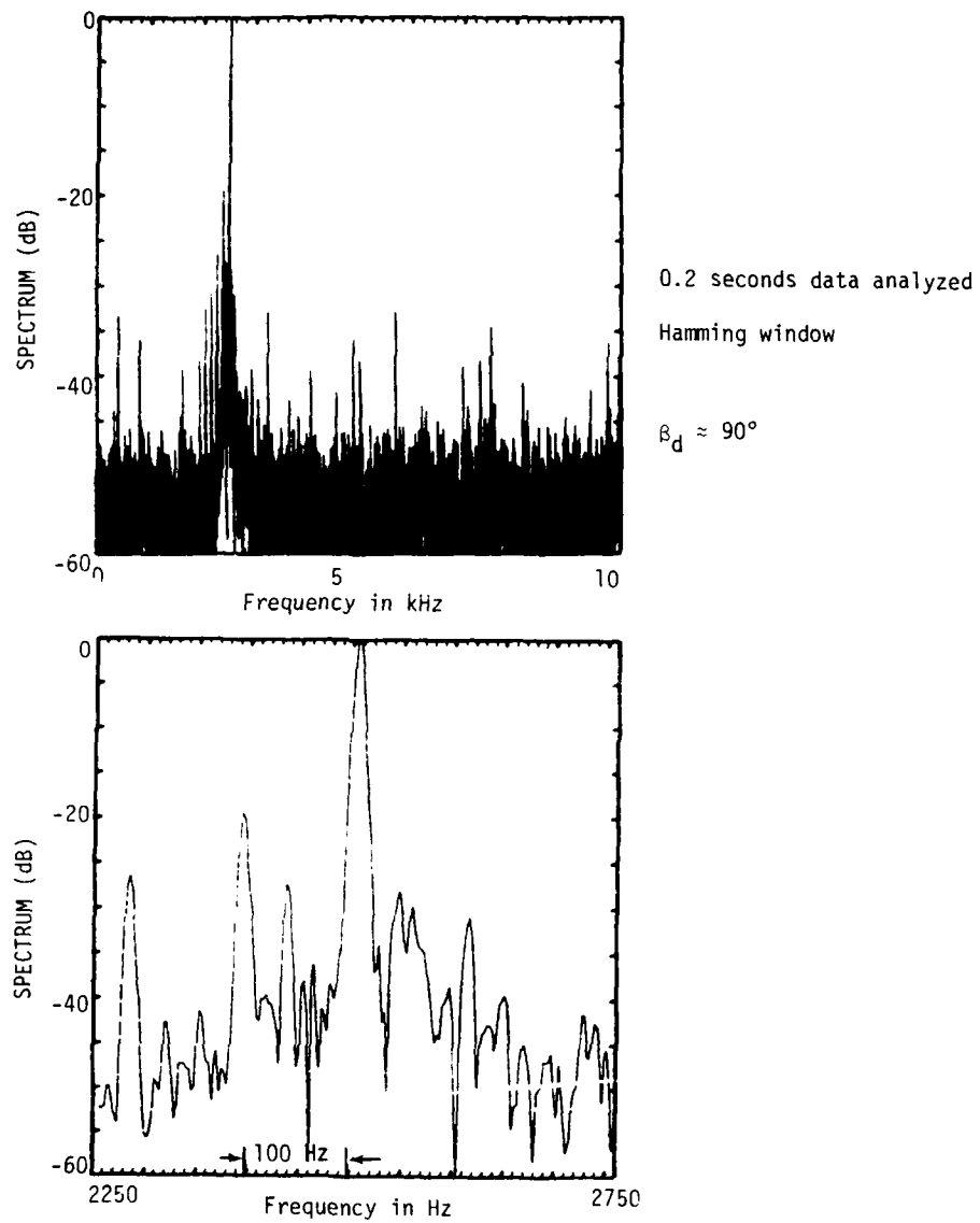
Fig. 3-42. Hanscom propeller modulation test.
