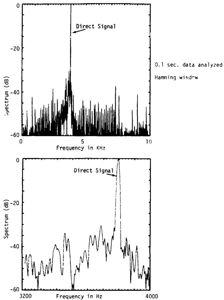
Fig.3-72. Spectrum of demodulated signal at WPAFB: example for low multipath region.
