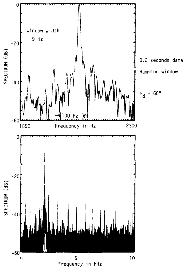
Fig. 3-41. Hanscom propeller modulation test spectrum.
