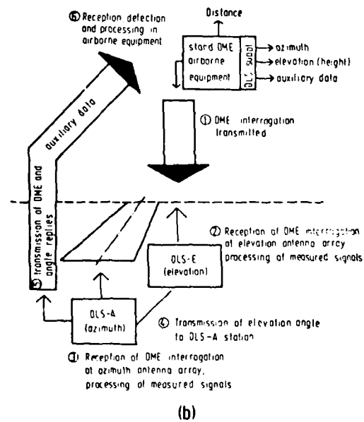
Fig.1-8(a-b). (a) Principle of the DME-based landing system DLS. (b) DLS signal flow.
