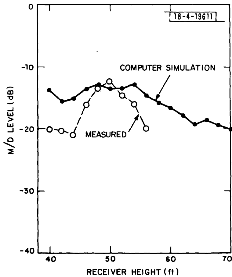
Fig.3-15. Comparison of measured and computed simulation predicted M/D levels for vertical cut at point C on JFK runway 13L centerline.
