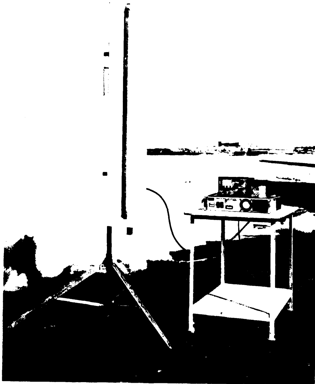
Fig. 3-25. MLS multipath measurement ground equipment.
