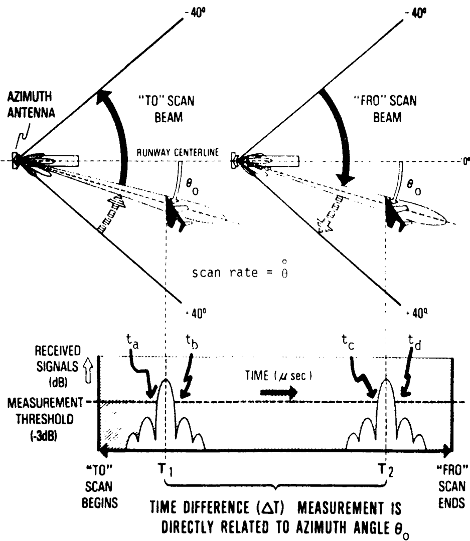
Fig.1-4. TRSB bi-direction scan format.
