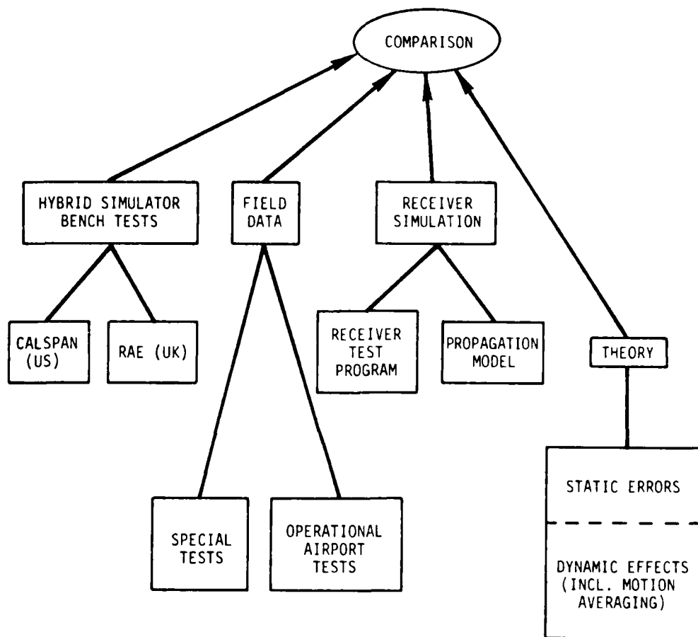
Fig.1-10. Elements of system model validation process.
