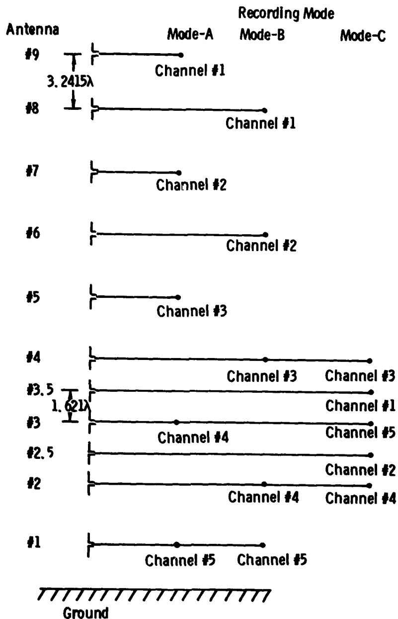
Fig.2-4. Relation of dipole antennas in the array to recording channels.
