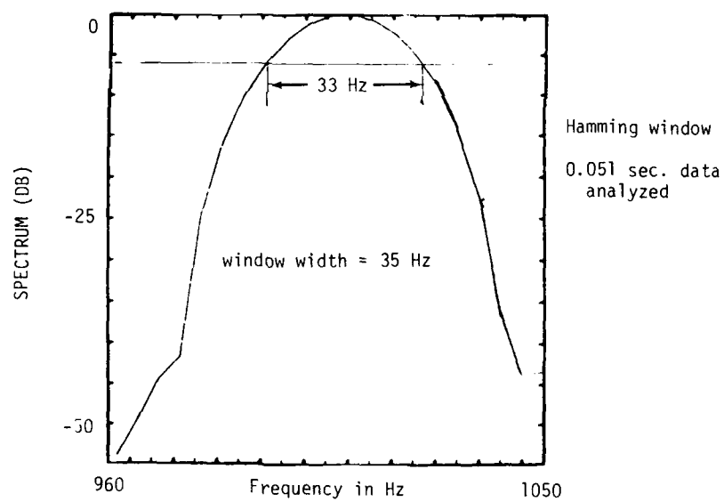
Fig.3-35. Spectrum of sinewave generator output.
