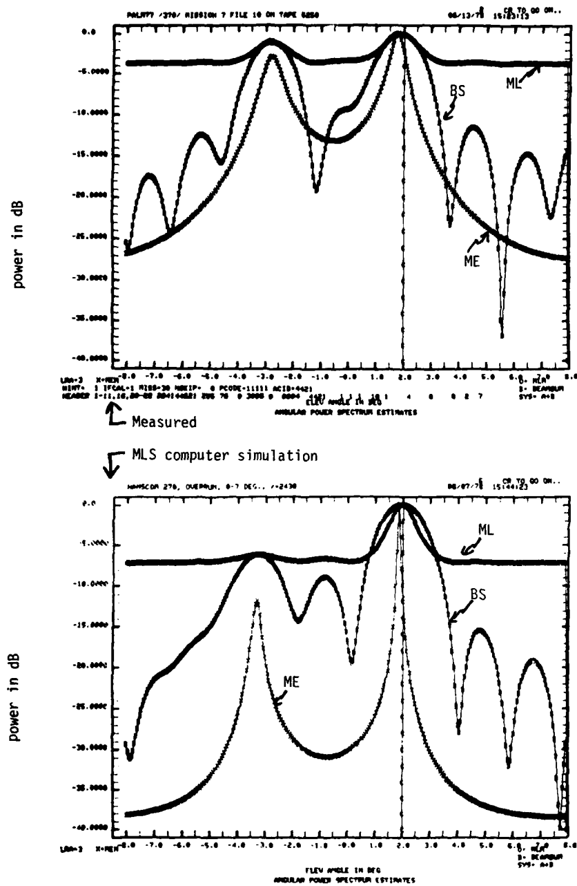
Fig. 2-24. Hanscom AFB measurements: \theta = 2.0^\circ .
