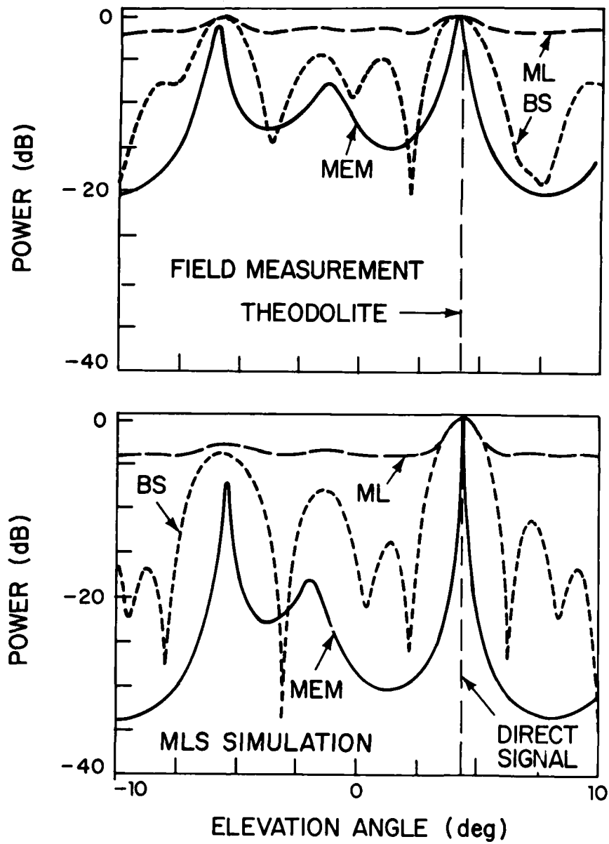
Fig. 2-31. Fort Devens measurement (golf course): \theta = 4.2^\circ .
