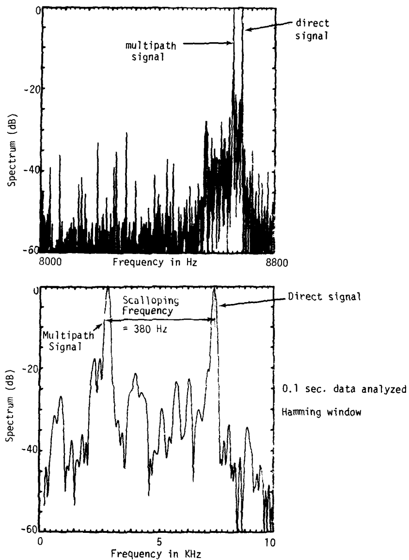
Fig. 3-74. Spectrum of demodulated signal: example of WPAFB multipath at 380 Hz scalloping frequency.
