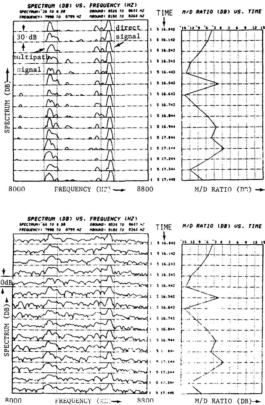
Fig. 3-75. WPAFB spectra on Run #3 at various points within the expected multipath region for building 206.
