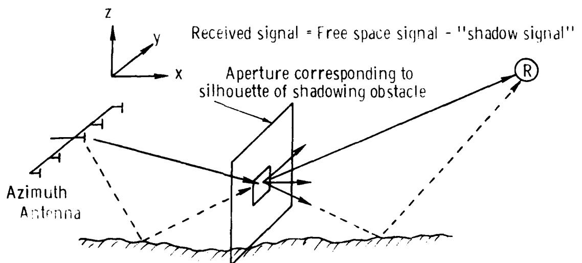
Fig.4-2. Huygen's principle applied to "shadowing signal" computation.
