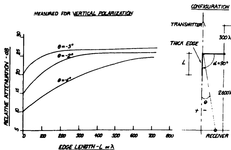
Fig. 4-24. Thick edge diffraction angles (from Oreb [80]).
