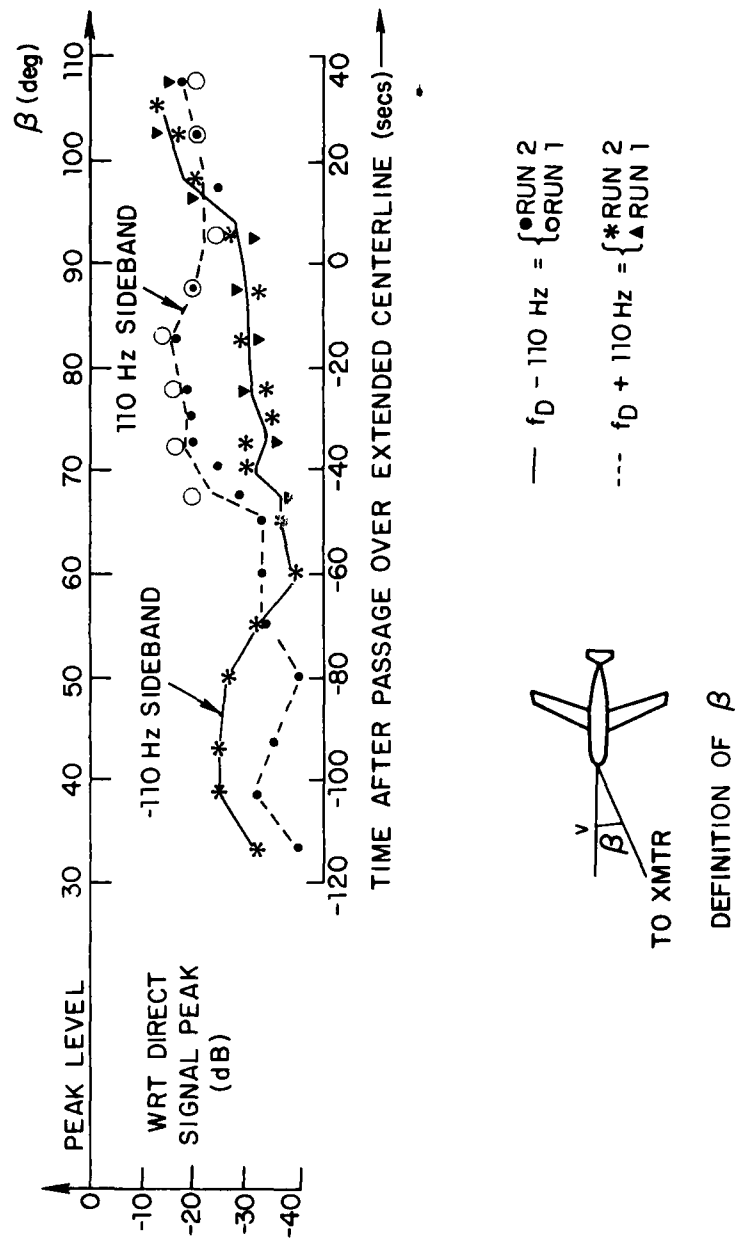
Fig. 3-43. Propeller modulation test sideband levels.
