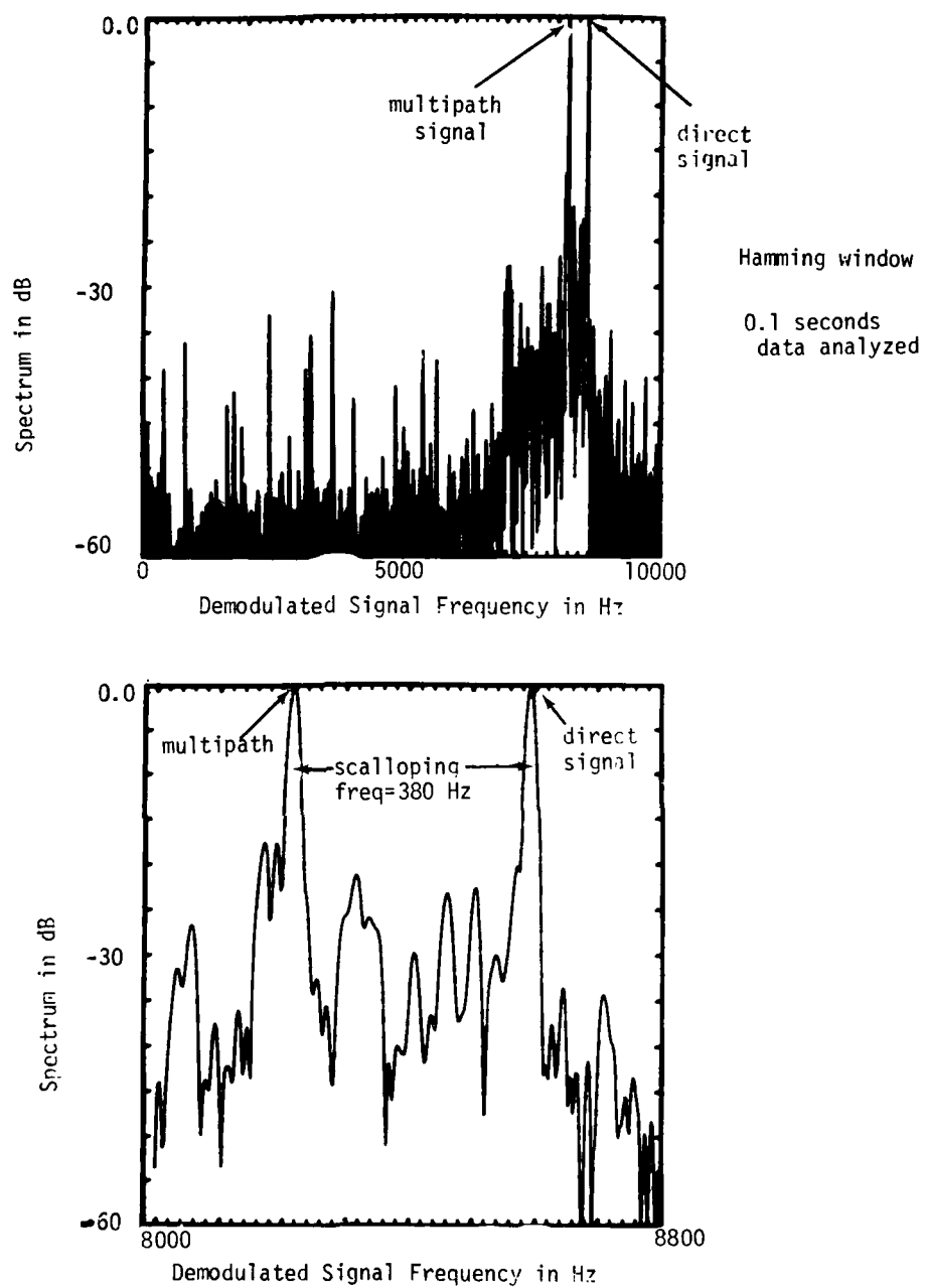
Fig.3-20. Spectrum of received signal at Wright Patterson AFB.
