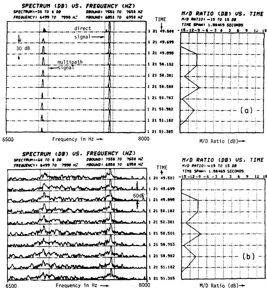
Fig.3-55. St.Louis spectra on run 3 at various points in expected multipath region for hangars 42 and 45.
