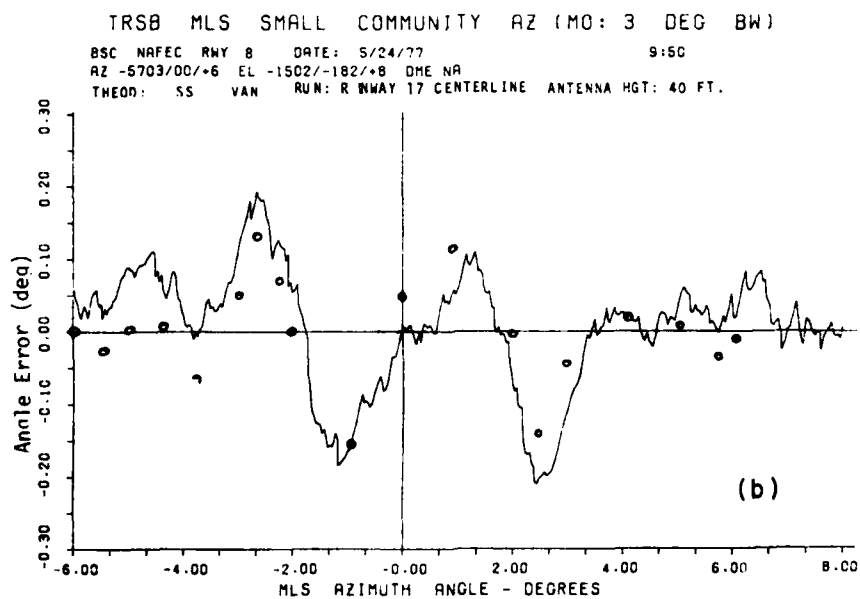
Fig.4-13(a-b). (a) TRSB angle error with normal monitor position. (b) Bendix small community TRSB azimuth errors with shadowing by monitor pole.
