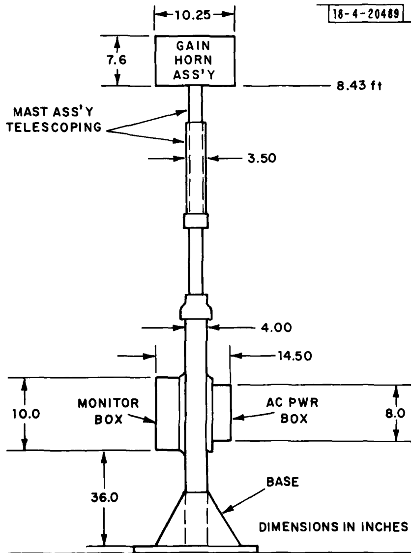
Fig. 4-11. Small community azimuth monitor.
