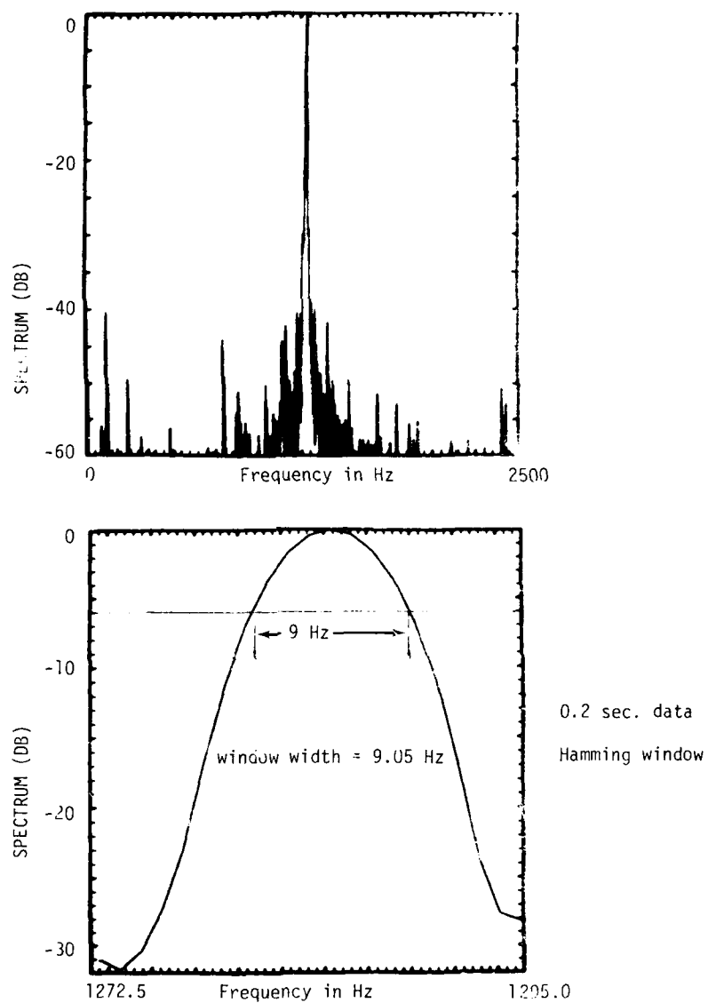
Fig.3-36. Spectrum of demodulated signal for bench test.
