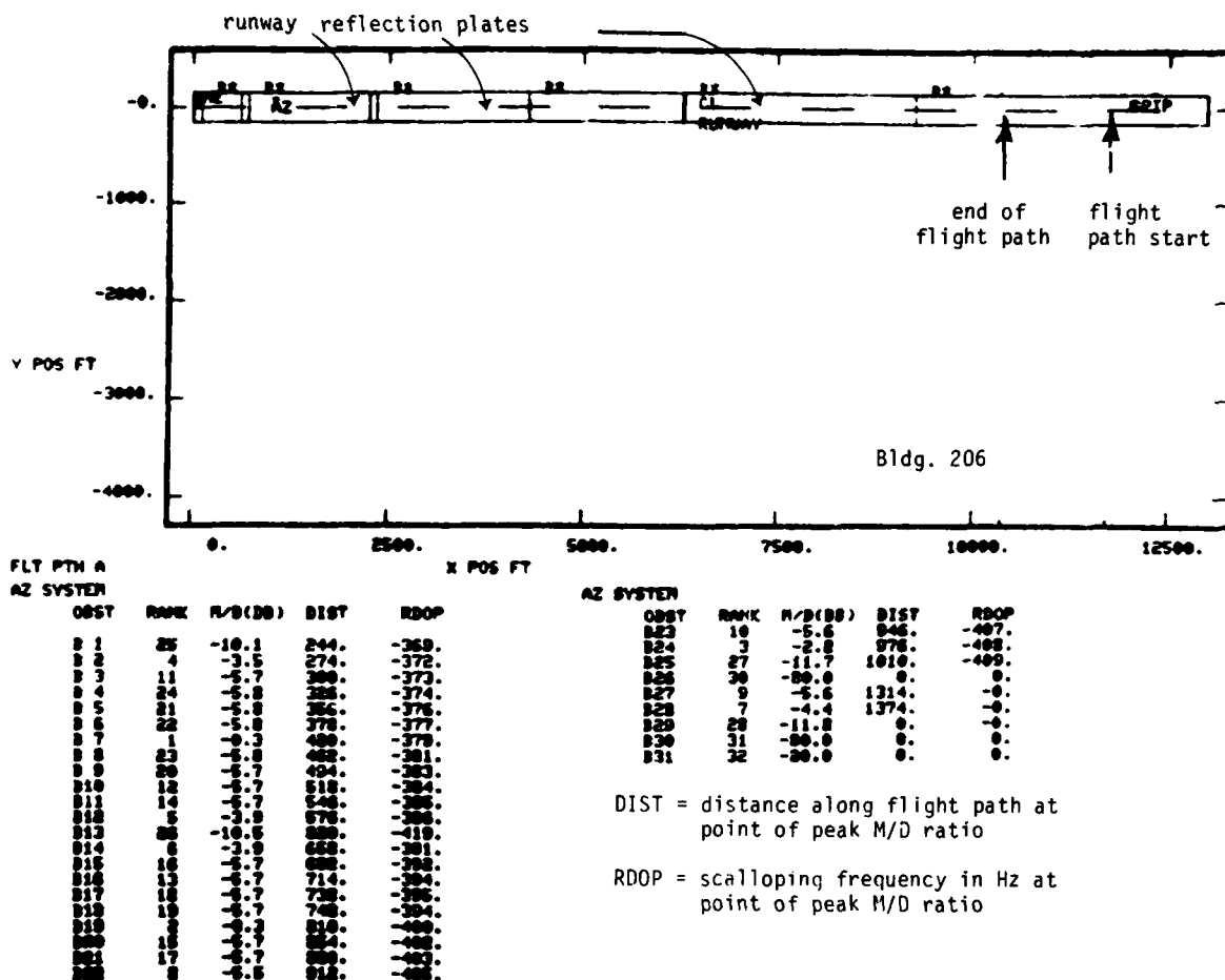
Fig.3-115. Airport map for simulation of WPAFB bldg. 206 reflections.
