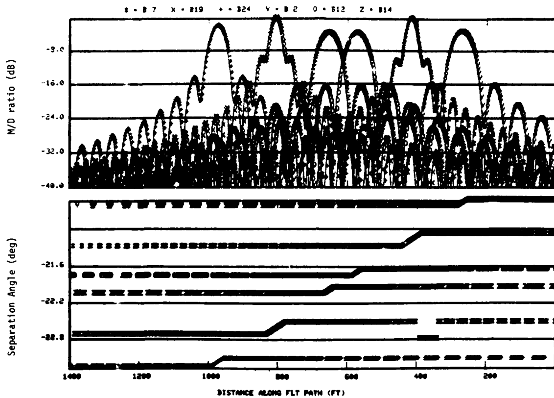
Fig.3-116. Computed multipath levels for six of WPAFB bldg. 206 doors.
