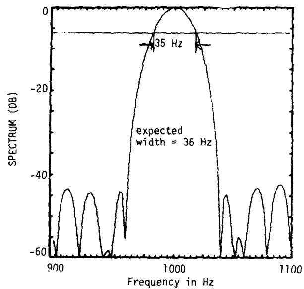
Fig.3-33. Hamming window applied to synthetic data.
