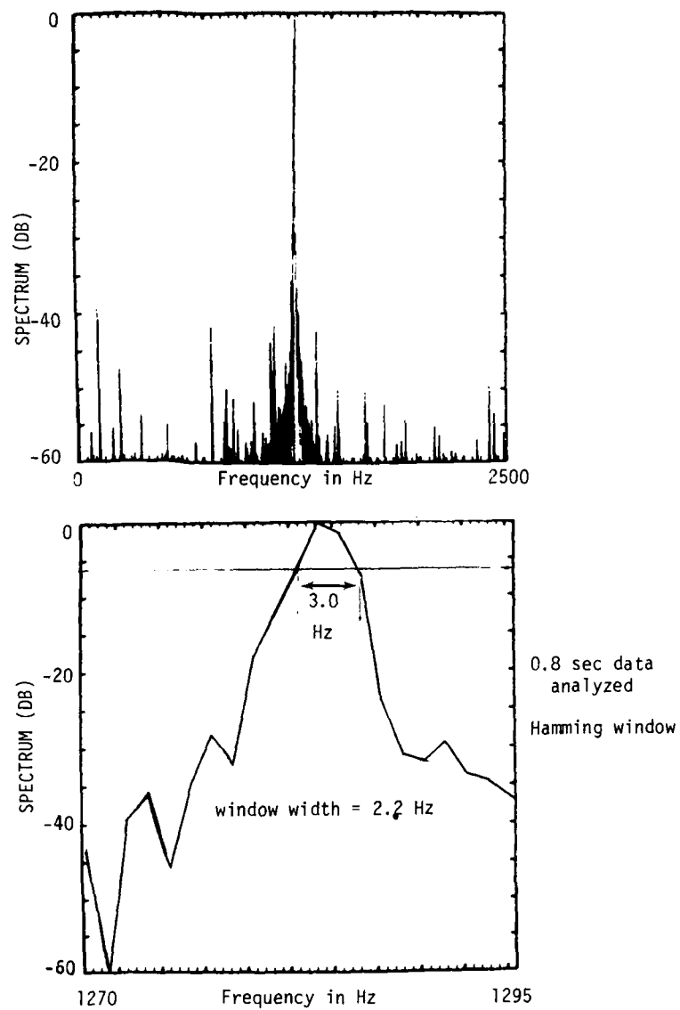
Fig.3-37. Demodulated signal spectrum for bench test.
