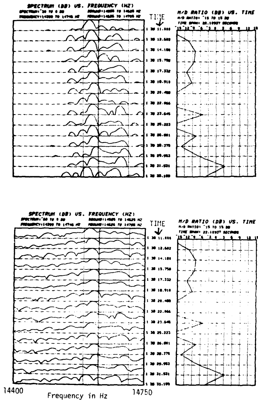
Fig. 3-91. Sequence of demodulated signal spectra for Miami run #7.
