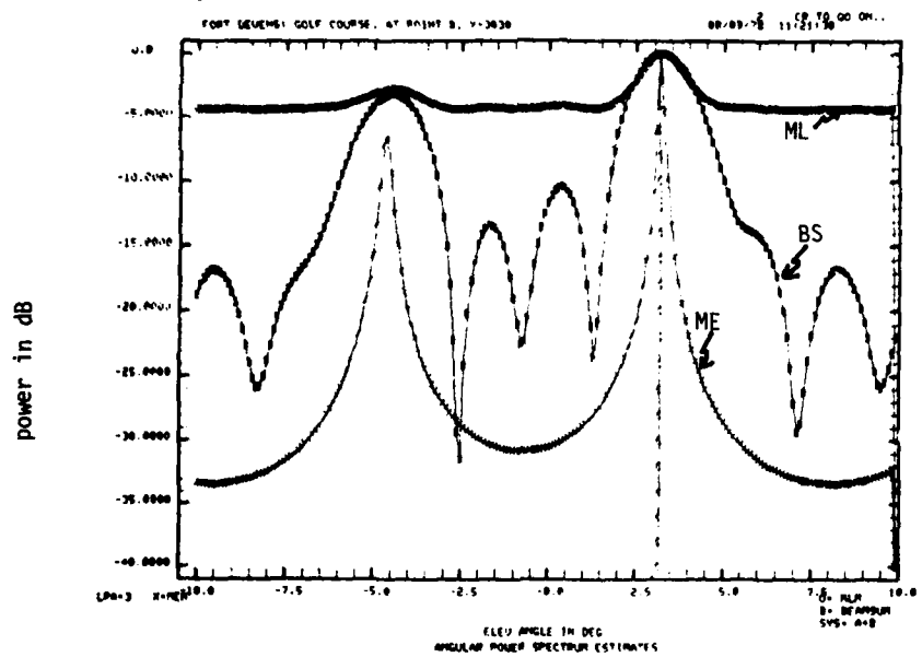
Fig. 2-30. Fort Devens measurement (golf course): \theta = 3.2^\circ .
