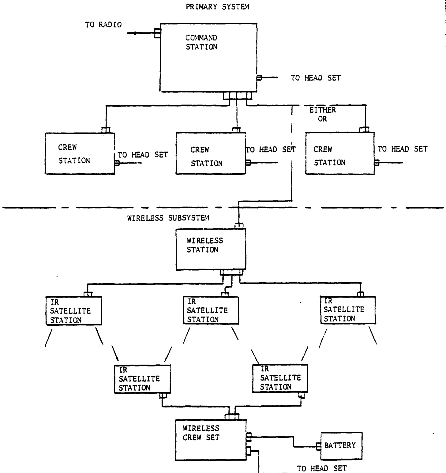
Figure 1. Block Diagram of Brassboard Test System
