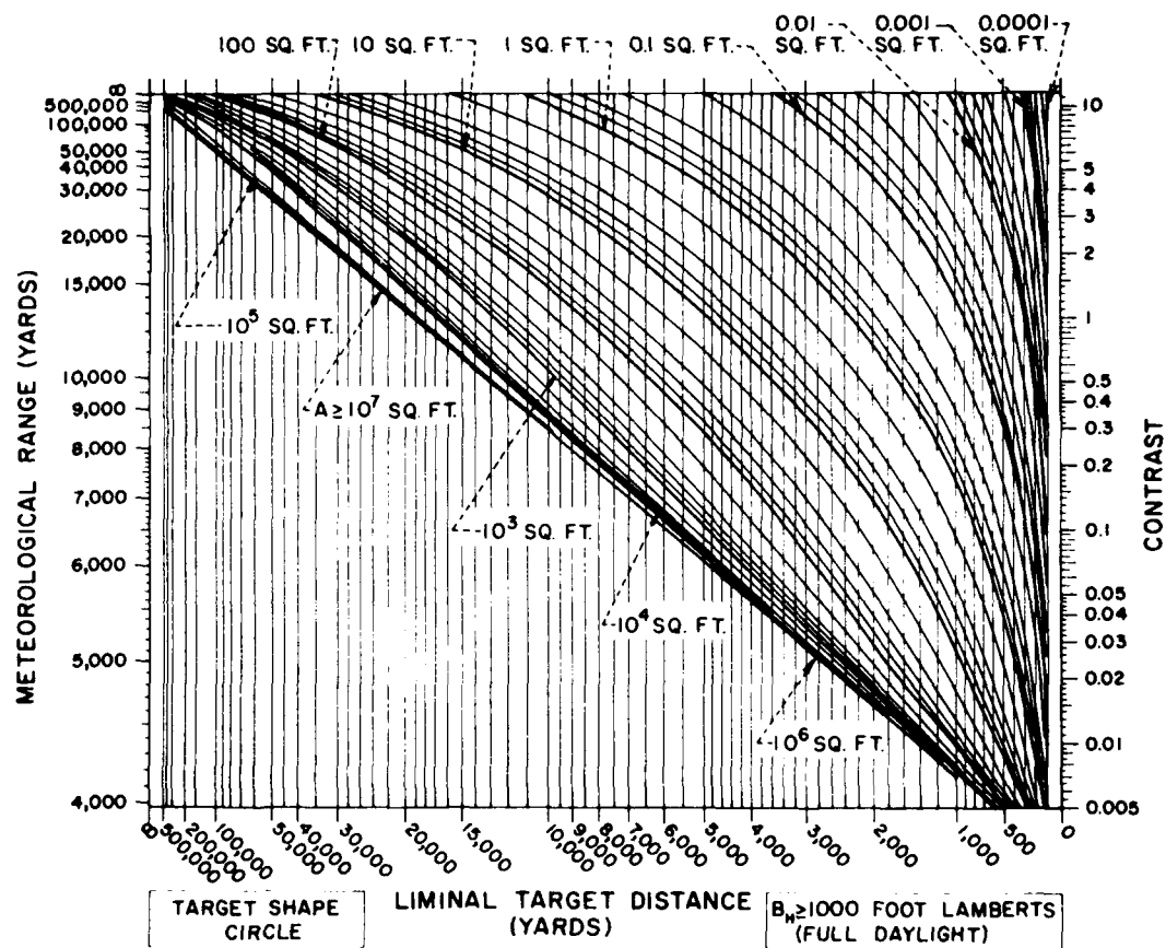
Figure 12. Nomograph for full daylight conditions (64, p. 239).
