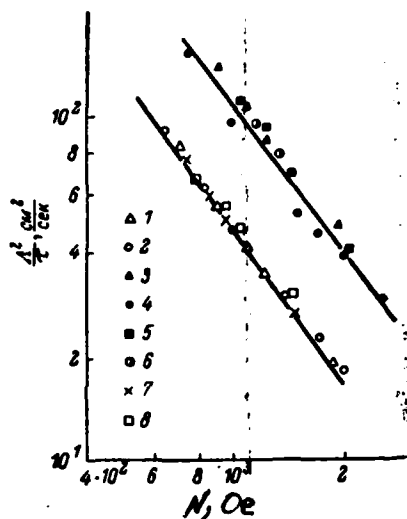
Figure 4. a) \frac{\Delta^2}{v} = f(H) - uniform magnetic field ( \delta < 6^\circ ), p = 0.04-0.05 Hg. 1 - data from the present study; 2 - data from work [6], p = 0.35-0.4 mm Hg; 3 - data from the present study; 4 - data from work [6]; b) p = 0.4 mm Hg
