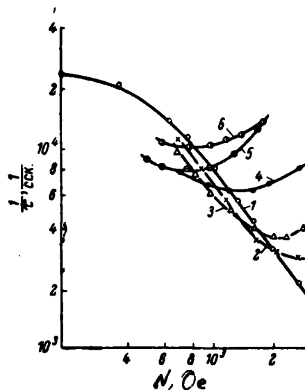
Figure 6 1 - p = 0.9 , 2 - 0.4, 3 - 0.12, 4 - 0.055, 5 - 0.04, 6 - 0.025 mm Hg
