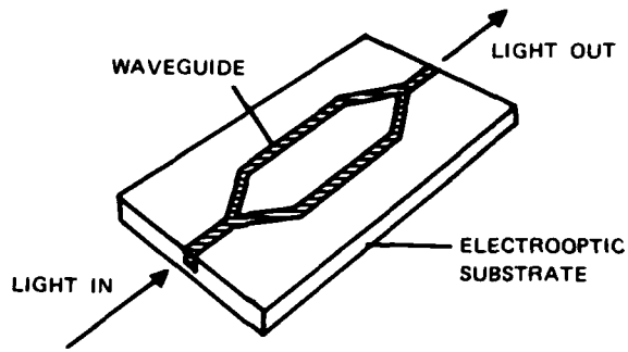
Figure 1. Basic interferometric modulator
