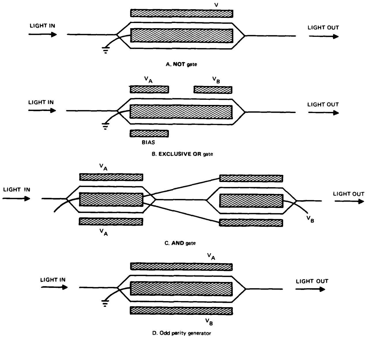
Figure 2. Device configuration.
