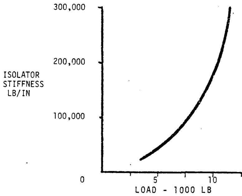
ISOLATOR REQUIREMENTS
