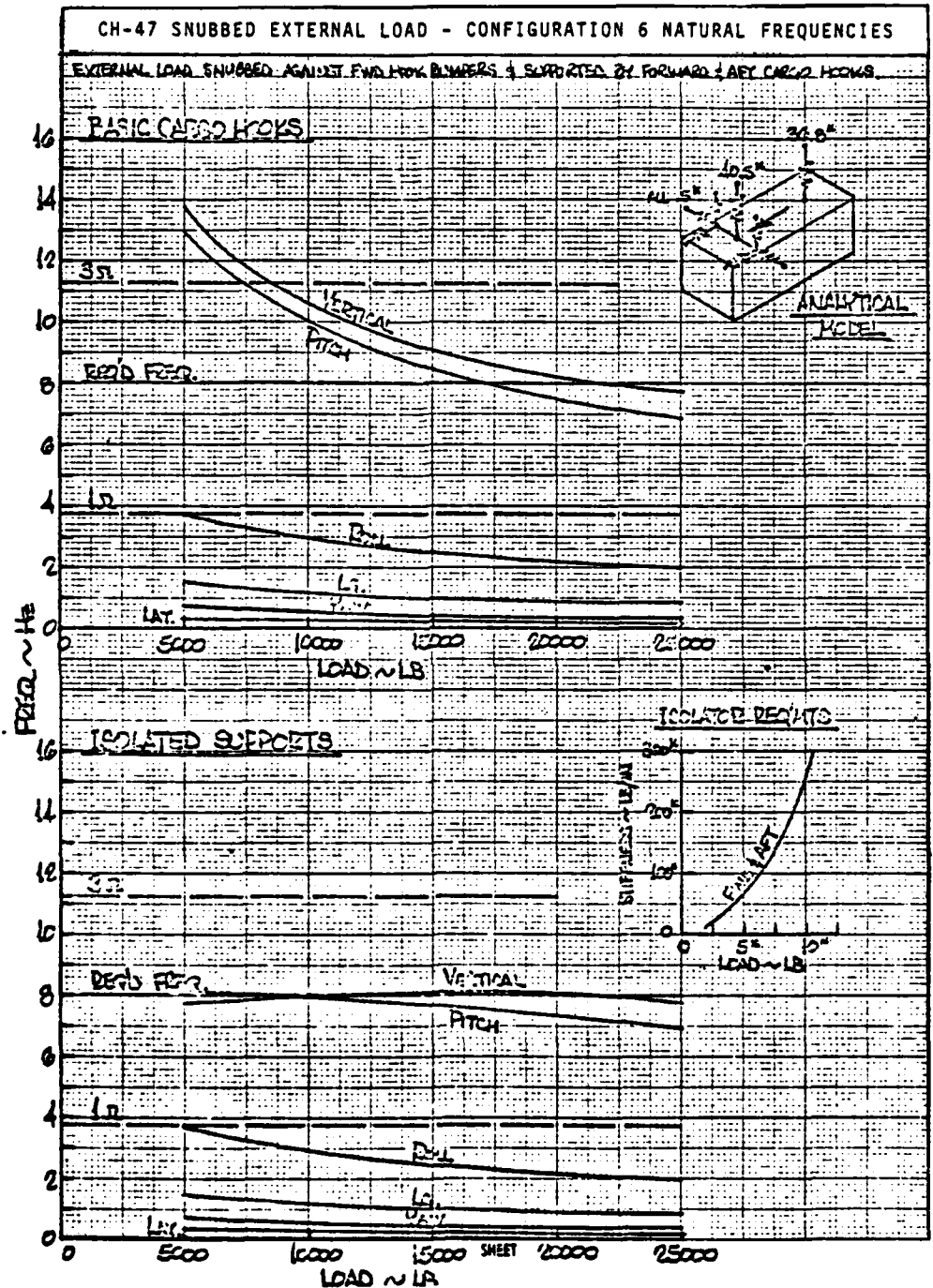
Figure 3.8 Effect of Support Isolation on Frequency Placement for Snubbed Load Configuration 6 (Tandem Hook + Bumpers on Frame)
