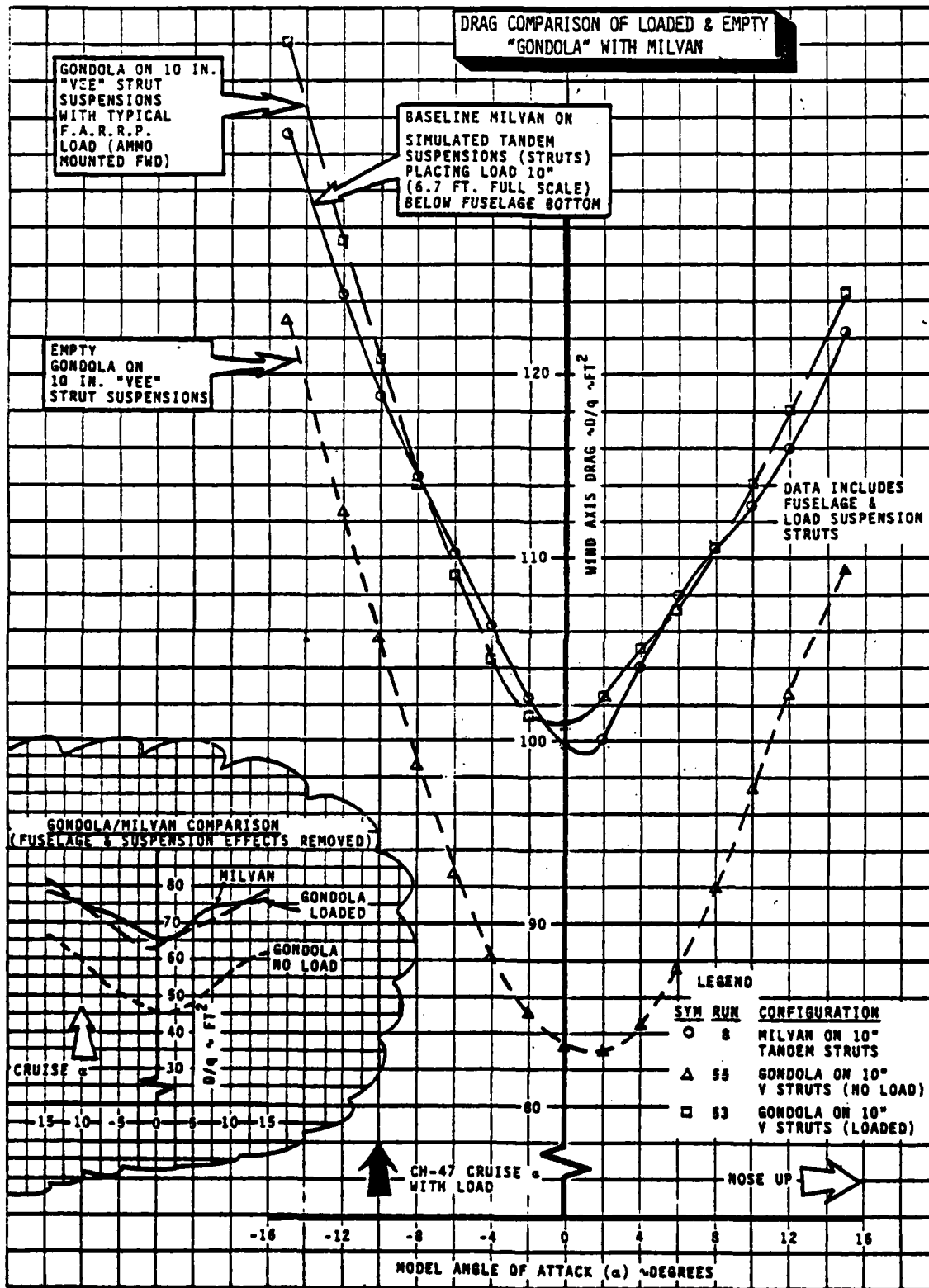
Figure 1.9 Gondola Drag
