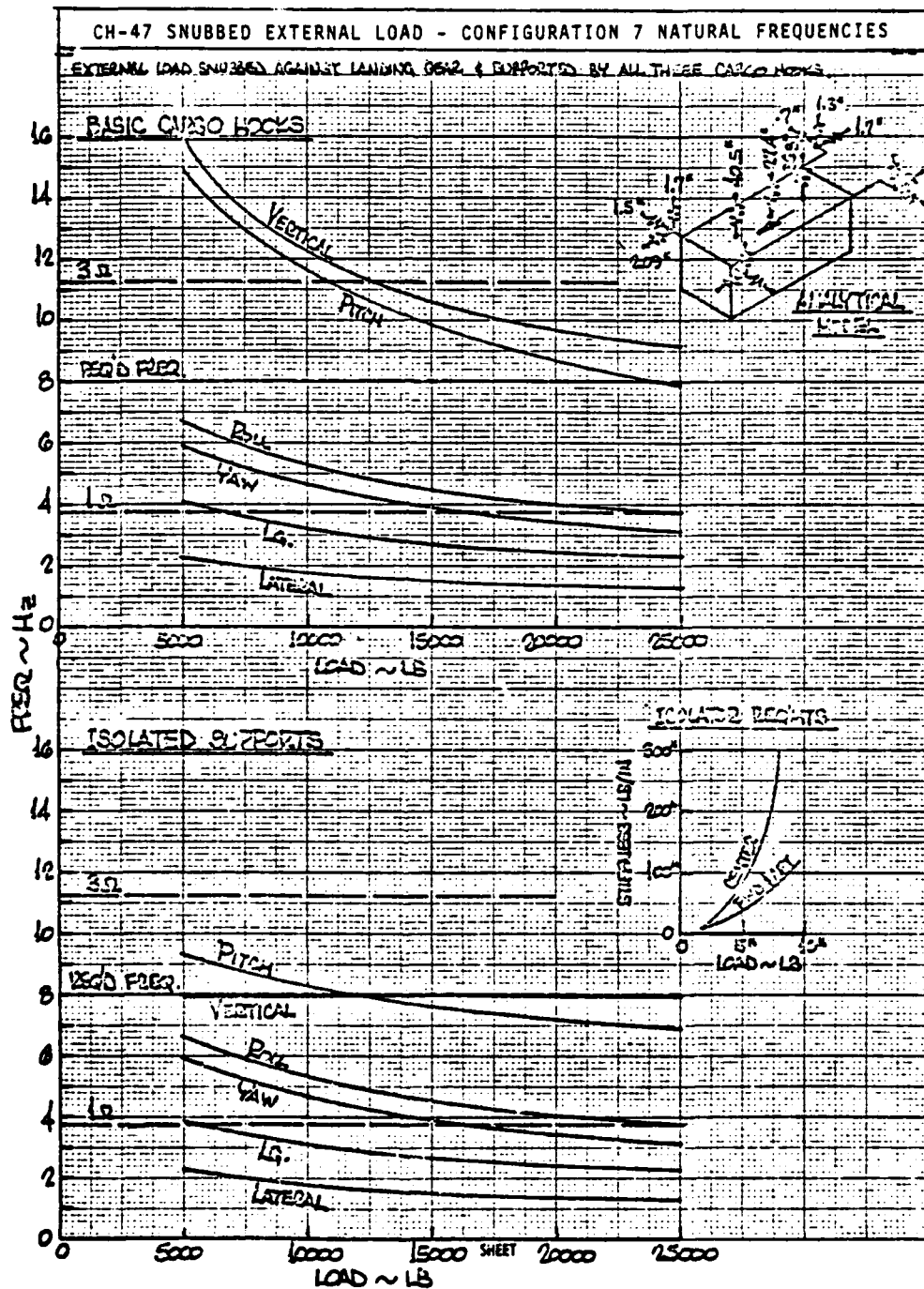
Figure 3.7 Effect of Support Isolation on Frequency Placement for Snubbed Load Configuration 7 (Three Hook Redundant)
