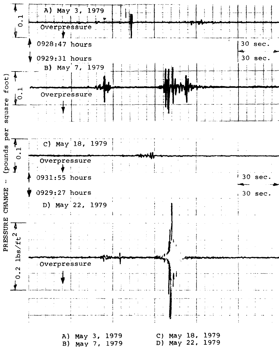
FIGURE 5. PRESSURE TIME HISTORIES SOURCE: BRITISH AIRWAYS FLIGHT BA-171 MALDEN MA
