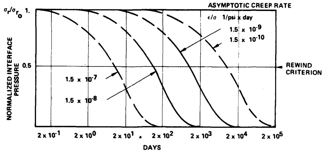
Figure 5 Basic trends of normalized interface pressure at hub vs. relaxation time. \sigma_{r0} is initial value of interface pressure. Solid lines are average values from Ref. [5], Figs. 4(a), 4(b). Broken lines are abstractions. Curves are based on a constant asymptotic creep rate.
